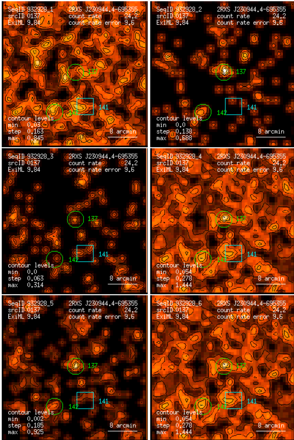
Figure 137: RASS 932928: detection 0137: band rate images, Gaussian filter: (1) PSPC channels 11 – 41, (2) 52 – 90, (3) 91 – 201, (4) 11 – 235, (5) 52 – 201, (6) 11 – 201. Broad band rates in counts/ks. Band rate contour levels in counts/ks/arcmin 2 .
