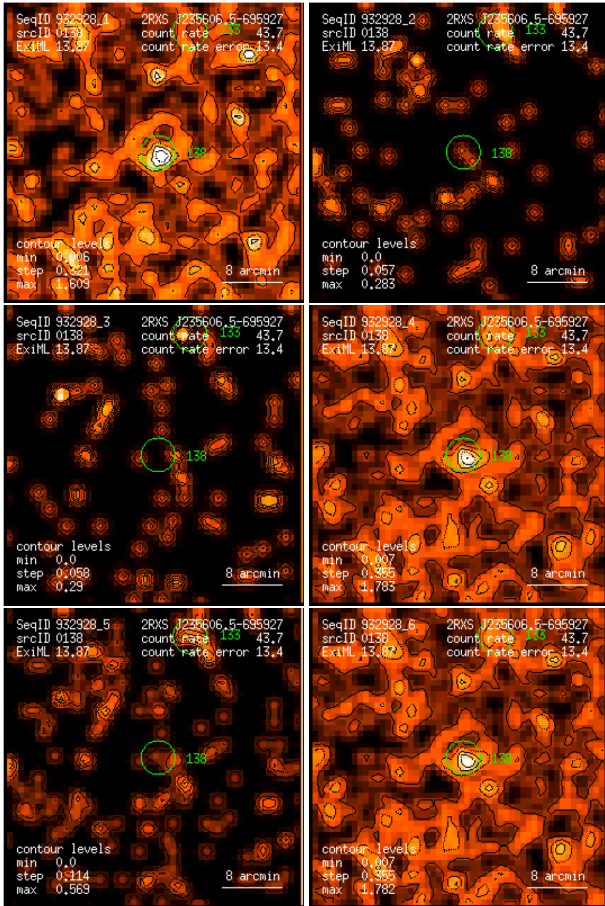
Figure 138: RASS 932928: detection 0138: band rate images, Gaussian filter: (1) PSPC channels 11 – 41, (2) 52 – 90, (3) 91 – 201, (4) 11 – 235, (5) 52 – 201, (6) 11 – 201. Broad band rates in counts/ks. Band rate contour levels in counts/ks/arcmin 2 .
