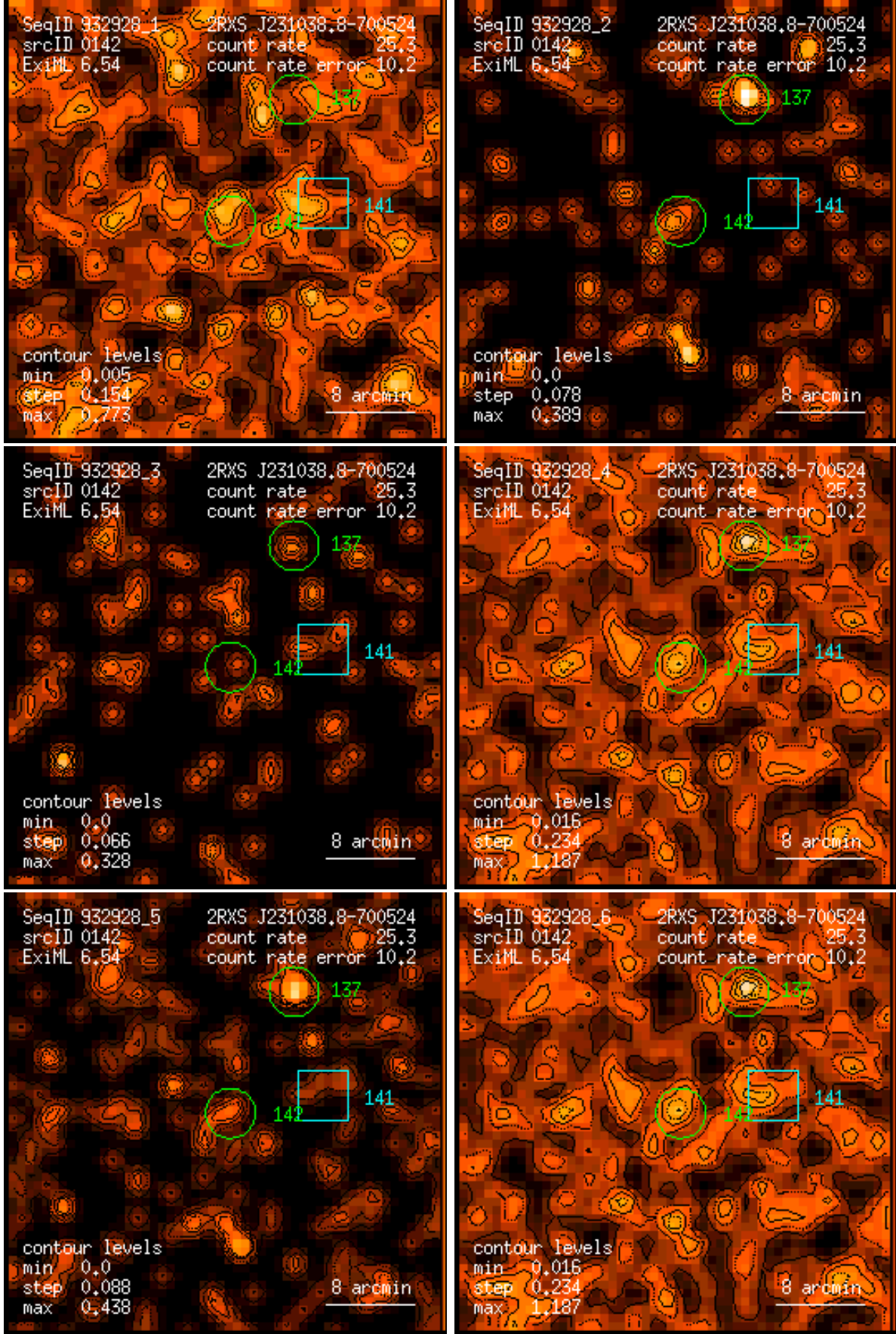
Figure 142: RASS 932928: detection 0142: band rate images, Gaussian filter: (1) PSPC channels 11 – 41, (2) 52 – 90, (3) 91 – 201, (4) 11 – 235, (5) 52 – 201, (6) 11 – 201. Broad band rates in counts/ks. Band rate contour levels in counts/ks/arcmin 2 .
