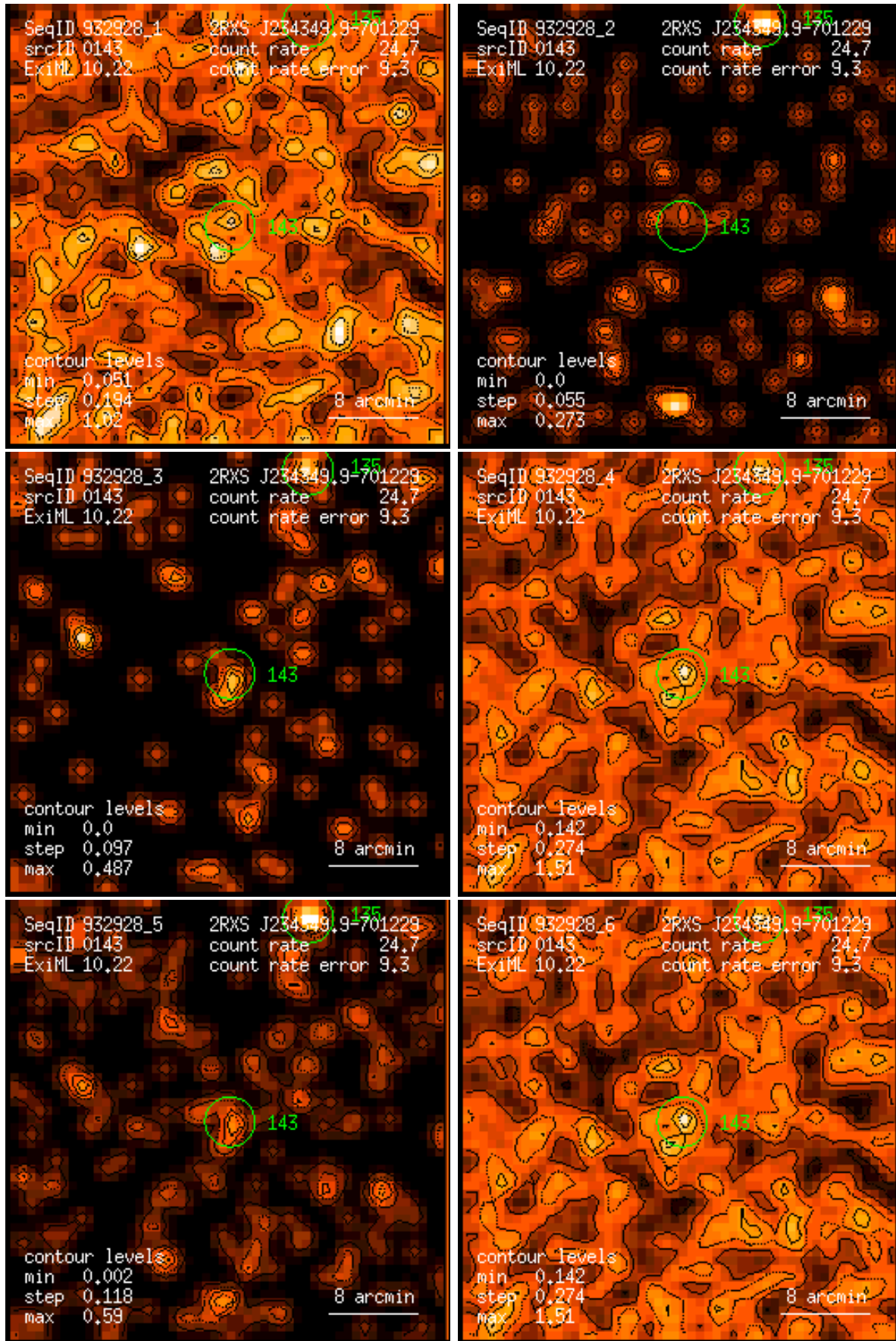
Figure 143: RASS 932928: detection 0143: band rate images, Gaussian filter: (1) PSPC channels 11 – 41, (2) 52 – 90, (3) 91 – 201, (4) 11 – 235, (5) 52 – 201, (6) 11 – 201. Broad band rates in counts/ks. Band rate contour levels in counts/ks/arcmin 2 .
