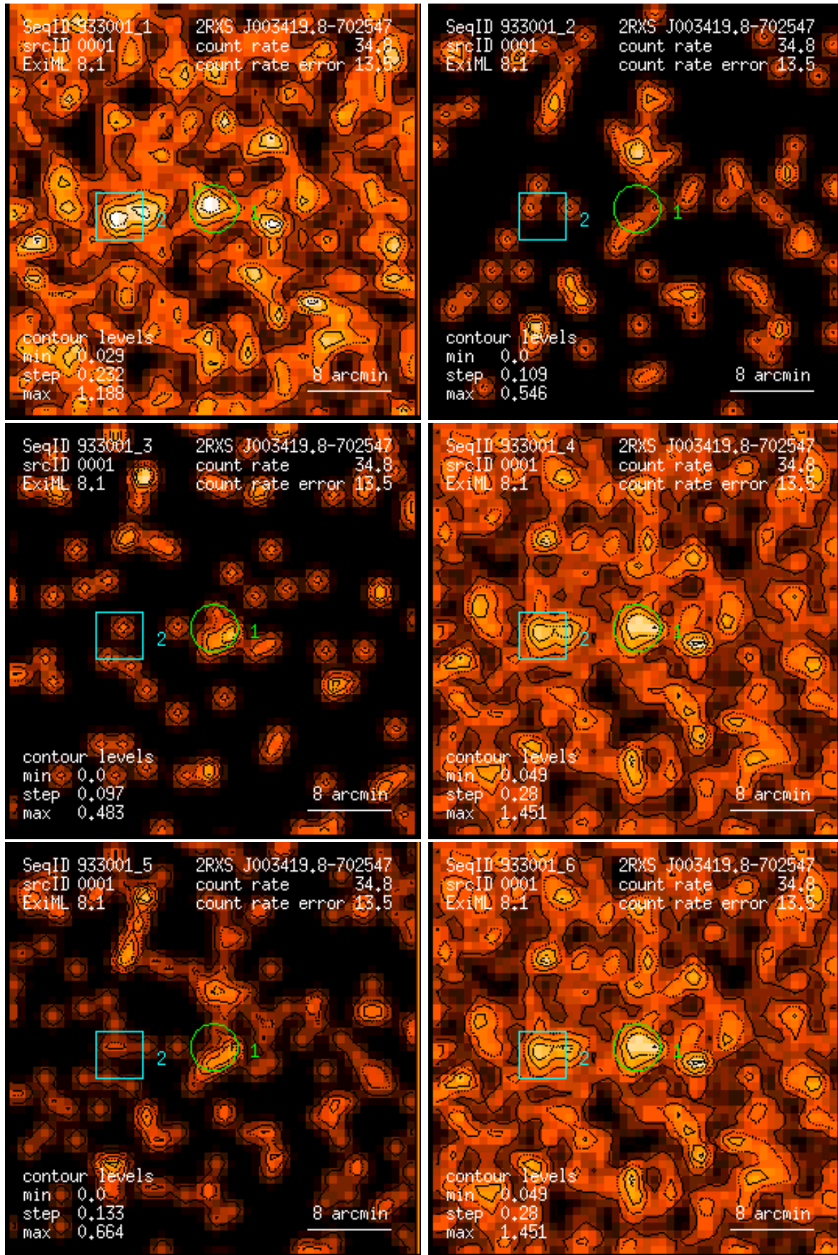
Figure 1: RASS 933001: detection 0001: band rate images, Gaussian filter: (1) PSPC channels 11 – 41, (2) 52 – 90, (3) 91 – 201, (4) 11 – 235, (5) 52 – 201, (6) 11 – 201. Broad band rates in counts/ks. Band rate contour levels in counts/ks/arcmin 2 .
