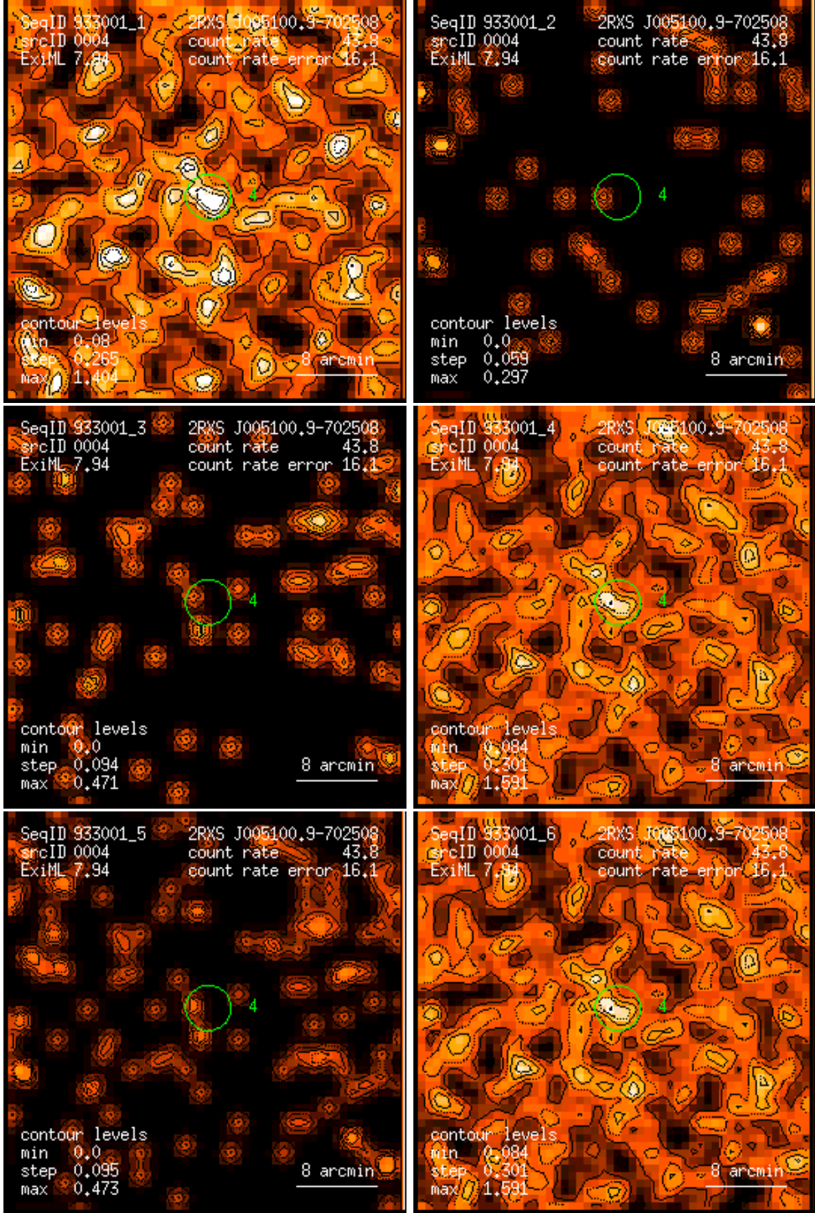
Figure 4: RASS 933001: detection 0004: band rate images, Gaussian filter: (1) PSPC channels 11 – 41, (2) 52 – 90, (3) 91 – 201, (4) 11 – 235, (5) 52 – 201, (6) 11 – 201. Broad band rates in counts/ks. Band rate contour levels in counts/ks/arcmin 2 .
