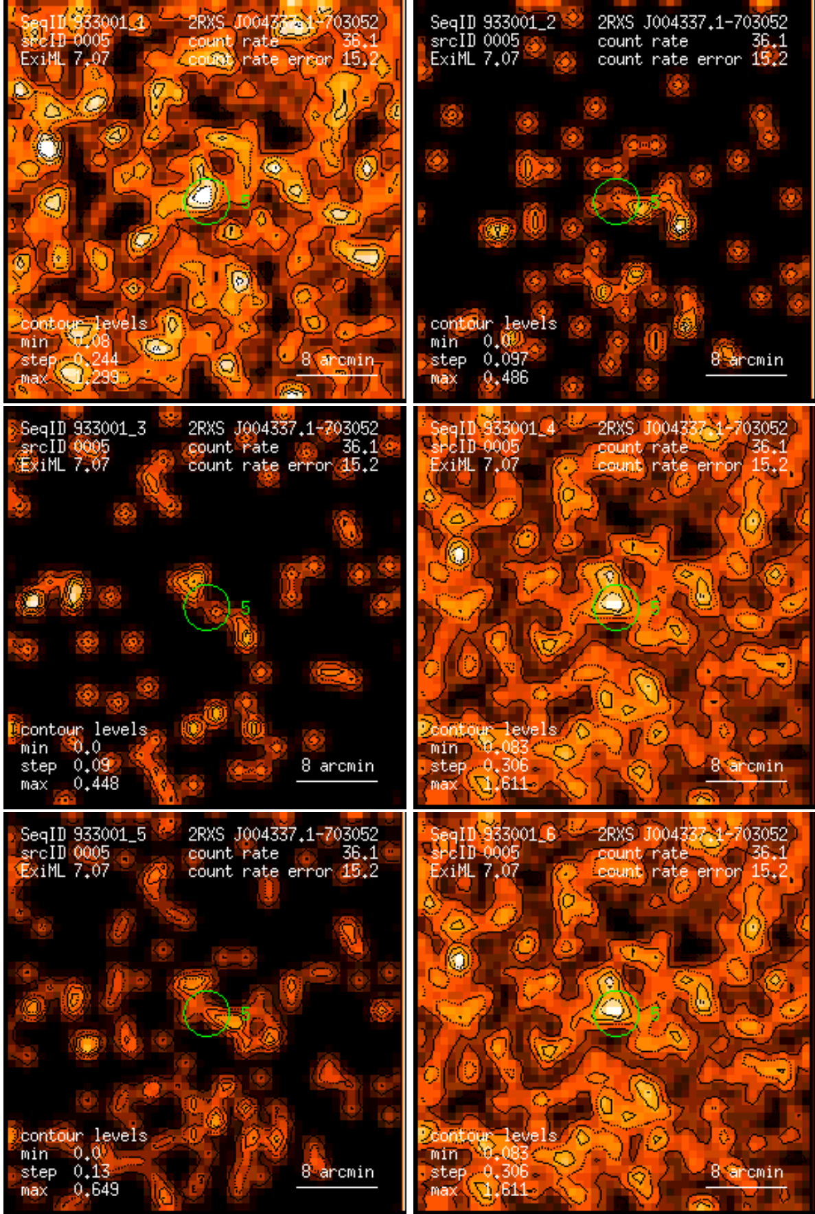
Figure 5: RASS 933001: detection 0005: band rate images, Gaussian filter: (1) PSPC channels 11 – 41, (2) 52 – 90, (3) 91 – 201, (4) 11 – 235, (5) 52 – 201, (6) 11 – 201. Broad band rates in counts/ks. Band rate contour levels in counts/ks/arcmin 2 .
