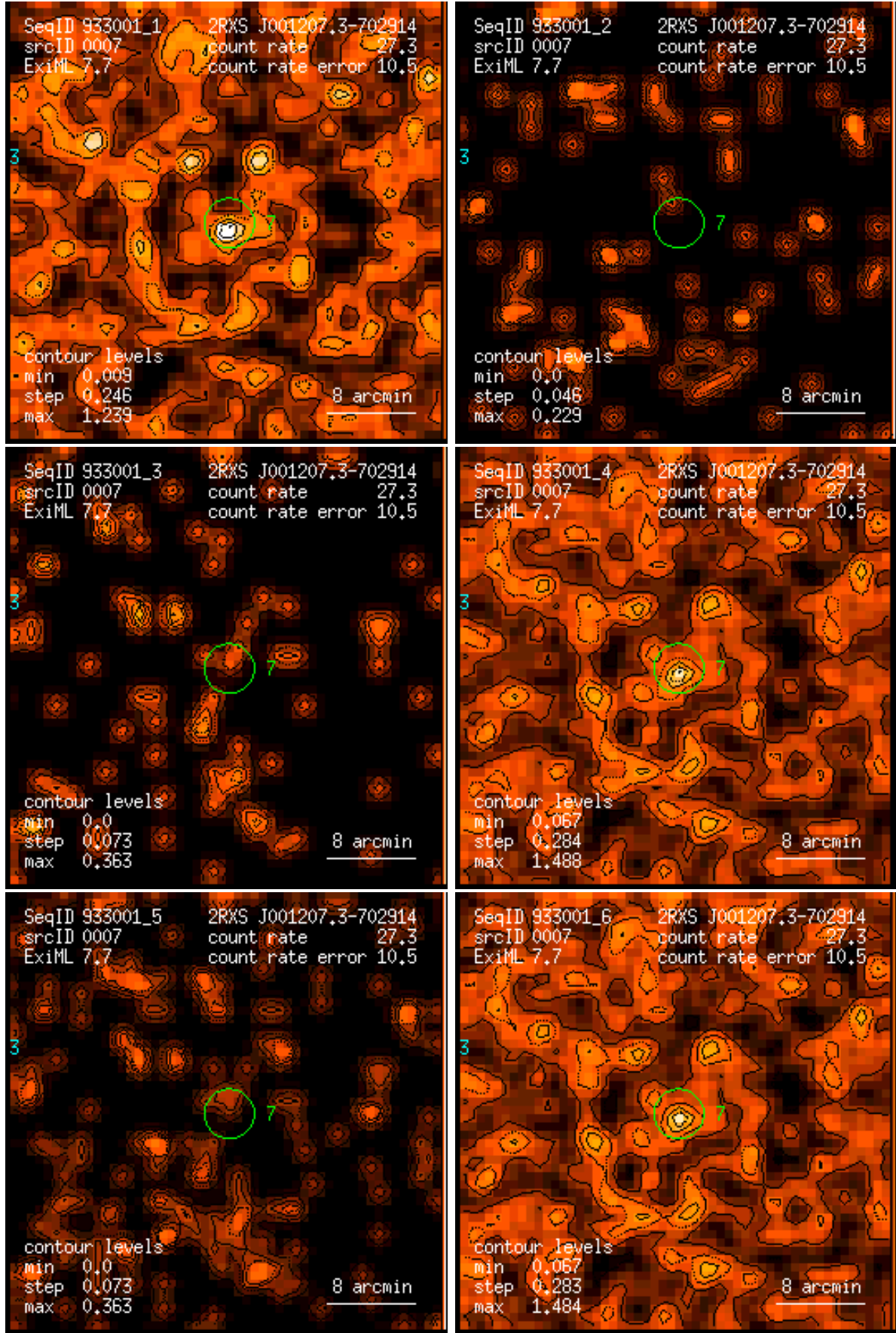
Figure 7: RASS 933001: detection 0007: band rate images, Gaussian filter: (1) PSPC channels 11 – 41, (2) 52 – 90, (3) 91 – 201, (4) 11 – 235, (5) 52 – 201, (6) 11 – 201. Broad band rates in counts/ks. Band rate contour levels in counts/ks/arcmin 2 .
