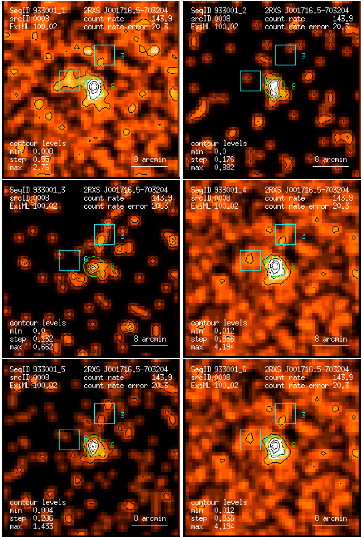
Figure 8: RASS 933001: detection 0008: band rate images, Gaussian filter: (1) PSPC channels 11 – 41, (2) 52 – 90, (3) 91 – 201, (4) 11 – 235, (5) 52 – 201, (6) 11 – 201. Broad band rates in counts/ks. Band rate contour levels in counts/ks/arcmin 2 .
