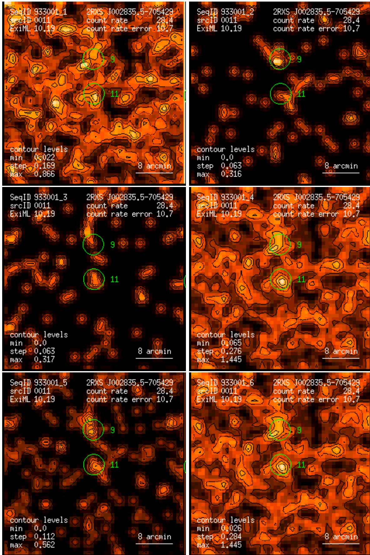
Figure 11: RASS 933001: detection 0011: band rate images, Gaussian filter: (1) PSPC channels 11 – 41, (2) 52 – 90, (3) 91 – 201, (4) 11 – 235, (5) 52 – 201, (6) 11 – 201. Broad band rates in counts/ks. Band rate contour levels in counts/ks/arcmin 2 .
