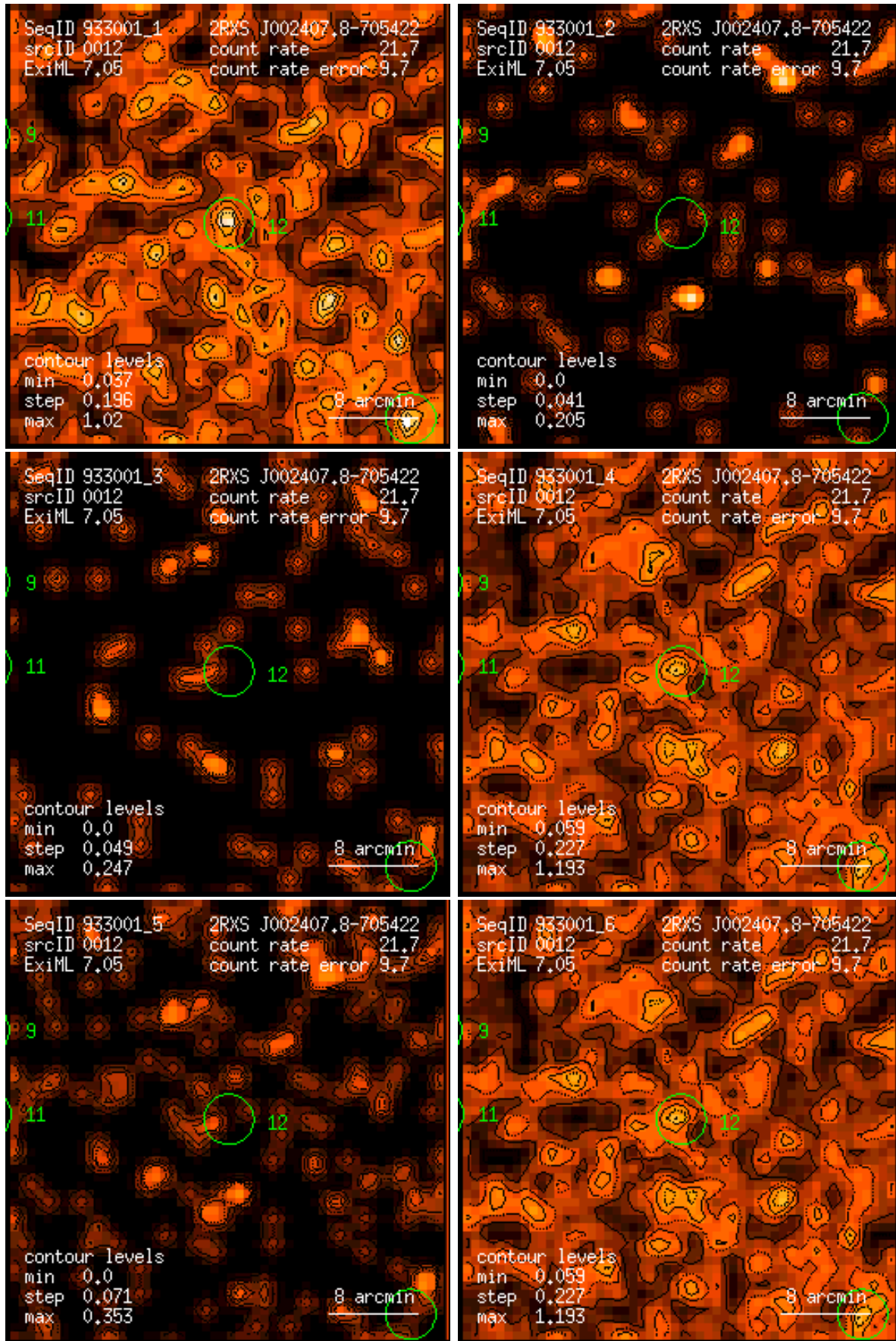
Figure 12: RASS 933001: detection 0012: band rate images, Gaussian filter: (1) PSPC channels 11 – 41, (2) 52 – 90, (3) 91 – 201, (4) 11 – 235, (5) 52 – 201, (6) 11 – 201. Broad band rates in counts/ks. Band rate contour levels in counts/ks/arcmin 2 .
