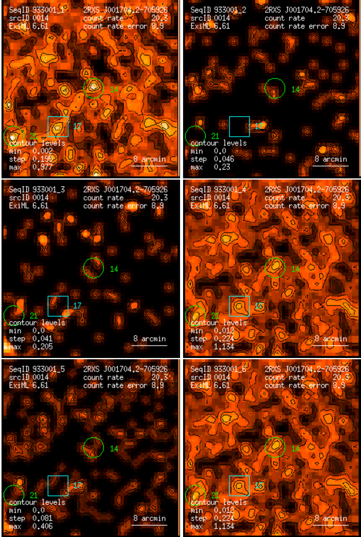
Figure 14: RASS 933001: detection 0014: band rate images, Gaussian filter: (1) PSPC channels 11 – 41, (2) 52 – 90, (3) 91 – 201, (4) 11 – 235, (5) 52 – 201, (6) 11 – 201. Broad band rates in counts/ks. Band rate contour levels in counts/ks/arcmin 2 .
