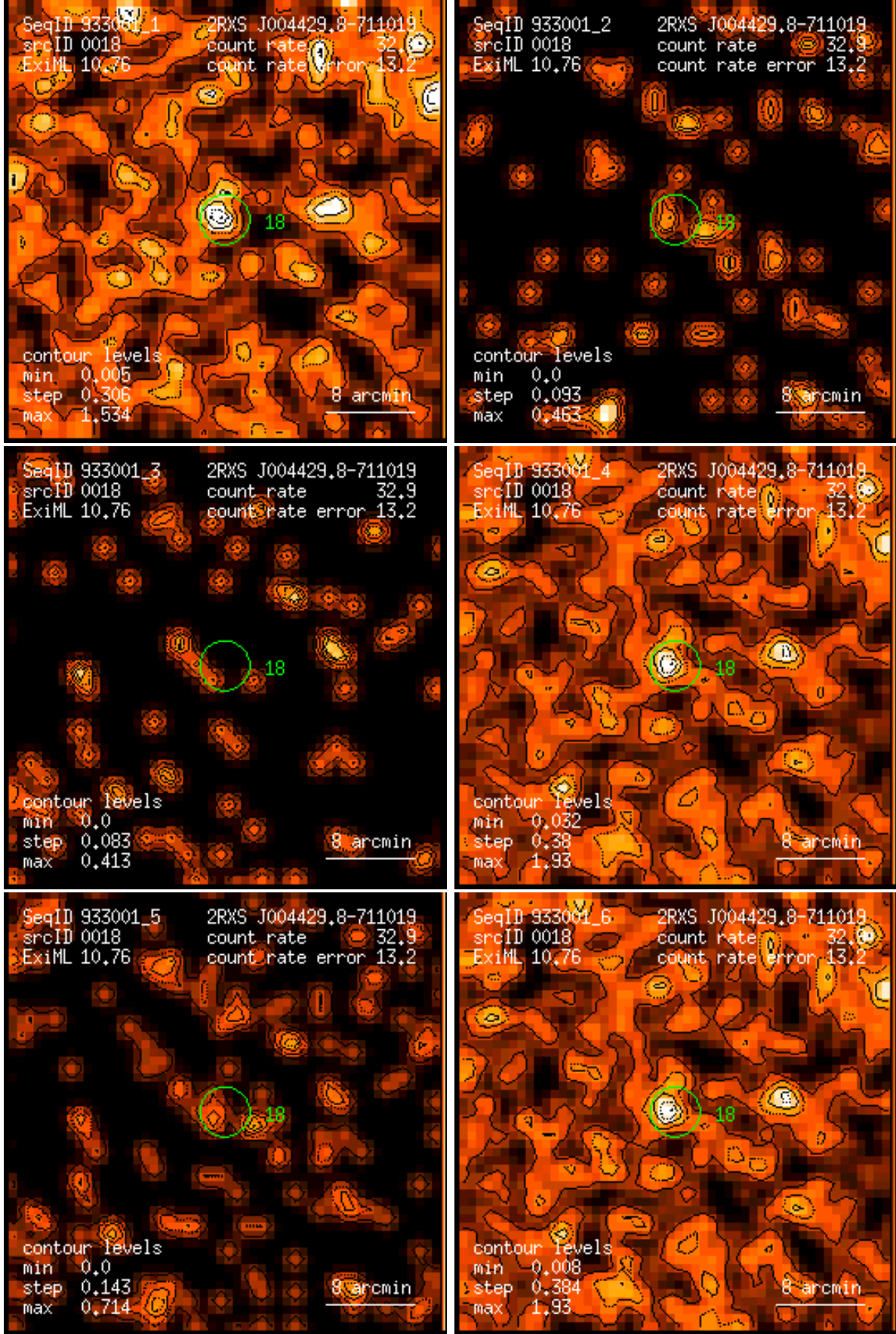
Figure 18: RASS 933001: detection 0018: band rate images, Gaussian filter: (1) PSPC channels 11 – 41, (2) 52 – 90, (3) 91 – 201, (4) 11 – 235, (5) 52 – 201, (6) 11 – 201. Broad band rates in counts/ks. Band rate contour levels in counts/ks/arcmin 2 .
