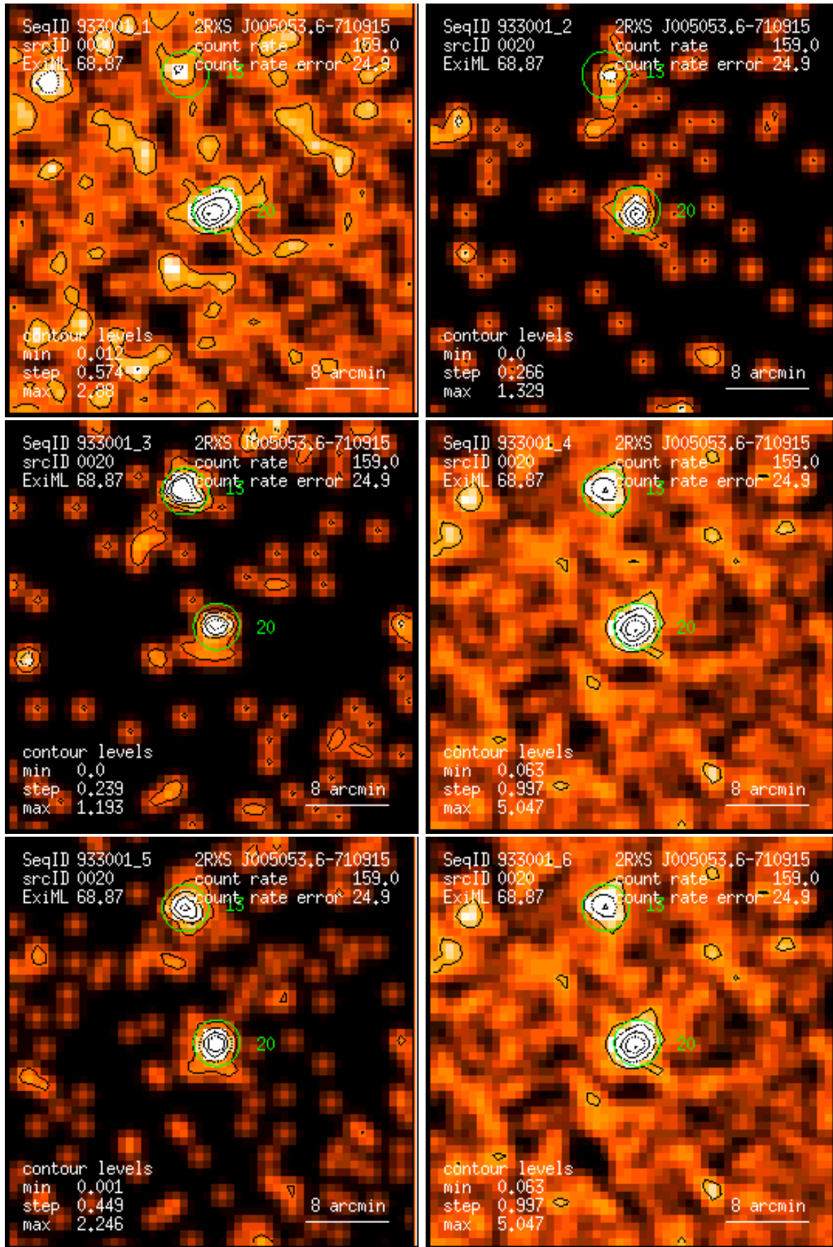
Figure 20: RASS 933001: detection 0020: band rate images, Gaussian filter: (1) PSPC channels 11 – 41, (2) 52 – 90, (3) 91 – 201, (4) 11 – 235, (5) 52 – 201, (6) 11 – 201. Broad band rates in counts/ks. Band rate contour levels in counts/ks/arcmin 2 .
