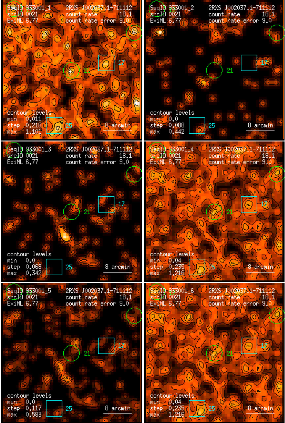
Figure 21: RASS 933001: detection 0021: band rate images, Gaussian filter: (1) PSPC channels 11 – 41, (2) 52 – 90, (3) 91 – 201, (4) 11 – 235, (5) 52 – 201, (6) 11 – 201. Broad band rates in counts/ks. Band rate contour levels in counts/ks/arcmin 2 .
