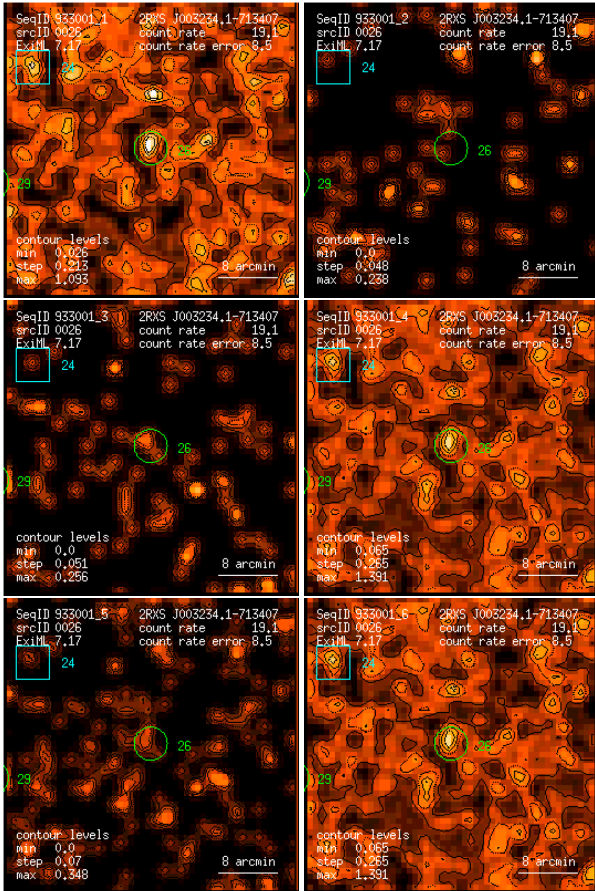
Figure 26: RASS 933001: detection 0026: band rate images, Gaussian filter: (1) PSPC channels 11 – 41, (2) 52 – 90, (3) 91 – 201, (4) 11 – 235, (5) 52 – 201, (6) 11 – 201. Broad band rates in counts/ks. Band rate contour levels in counts/ks/arcmin 2 .
