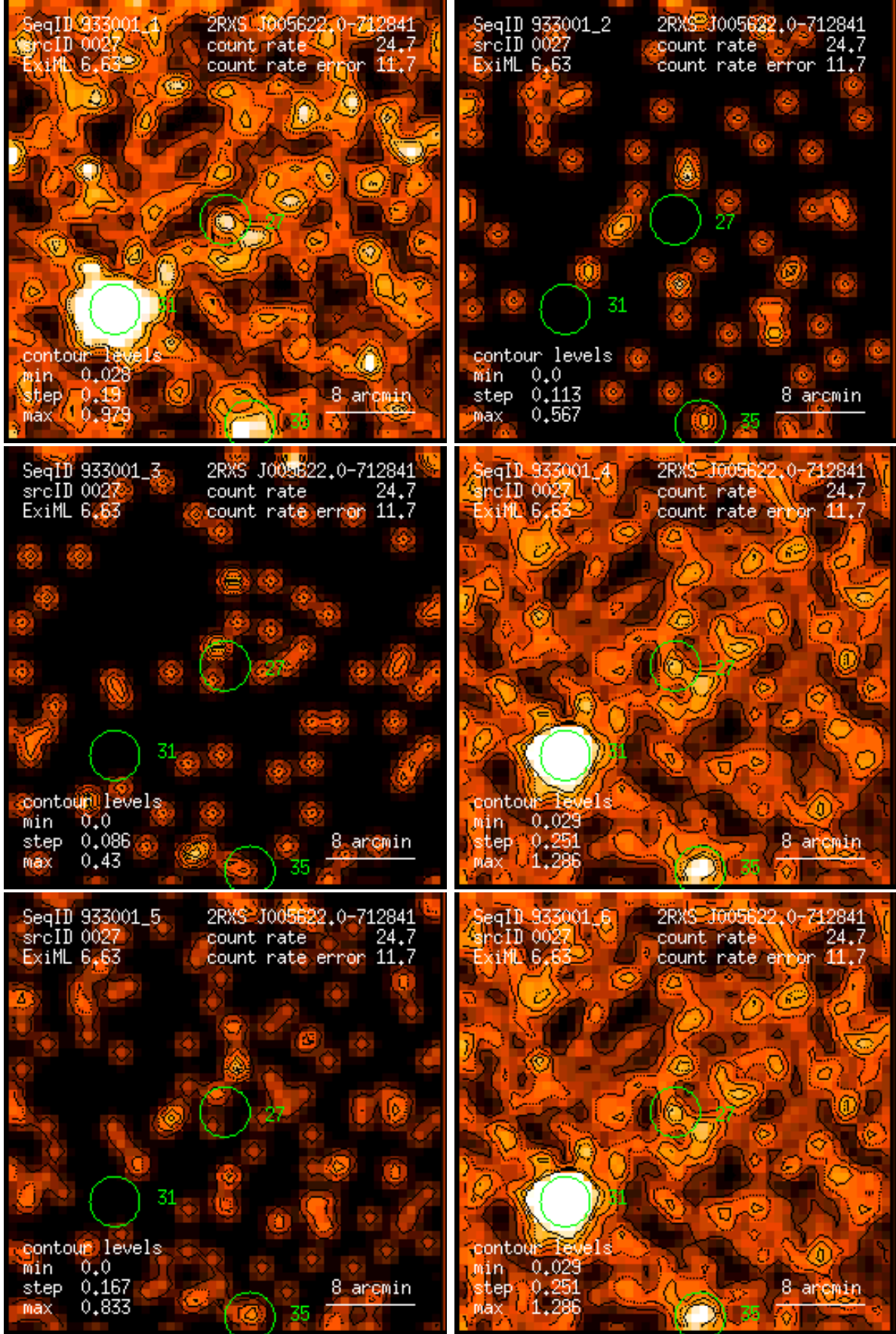
Figure 27: RASS 933001: detection 0027: band rate images, Gaussian filter: (1) PSPC channels 11 – 41, (2) 52 – 90, (3) 91 – 201, (4) 11 – 235, (5) 52 – 201, (6) 11 – 201. Broad band rates in counts/ks. Band rate contour levels in counts/ks/arcmin 2 .
