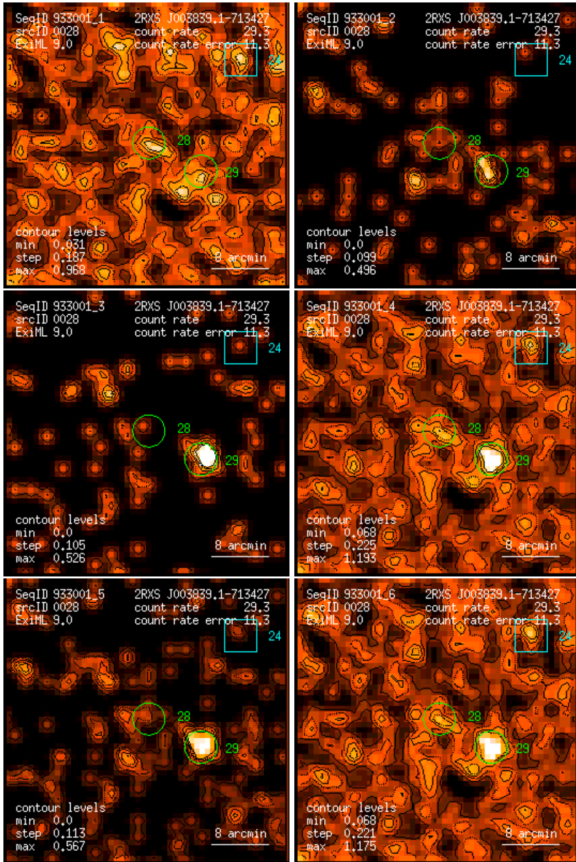
Figure 28: RASS 933001: detection 0028: band rate images, Gaussian filter: (1) PSPC channels 11 – 41, (2) 52 – 90, (3) 91 – 201, (4) 11 – 235, (5) 52 – 201, (6) 11 – 201. Broad band rates in counts/ks. Band rate contour levels in counts/ks/arcmin 2 .
