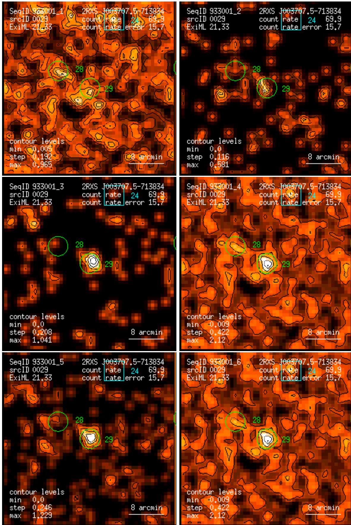
Figure 29: RASS 933001: detection 0029: band rate images, Gaussian filter: (1) PSPC channels 11 – 41, (2) 52 – 90, (3) 91 – 201, (4) 11 – 235, (5) 52 – 201, (6) 11 – 201. Broad band rates in counts/ks. Band rate contour levels in counts/ks/arcmin 2 .
