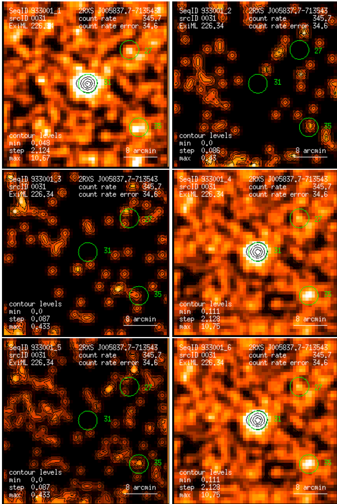
Figure 31: RASS 933001: detection 0031: band rate images, Gaussian filter: (1) PSPC channels 11 – 41, (2) 52 – 90, (3) 91 – 201, (4) 11 – 235, (5) 52 – 201, (6) 11 – 201. Broad band rates in counts/ks. Band rate contour levels in counts/ks/arcmin 2 .
