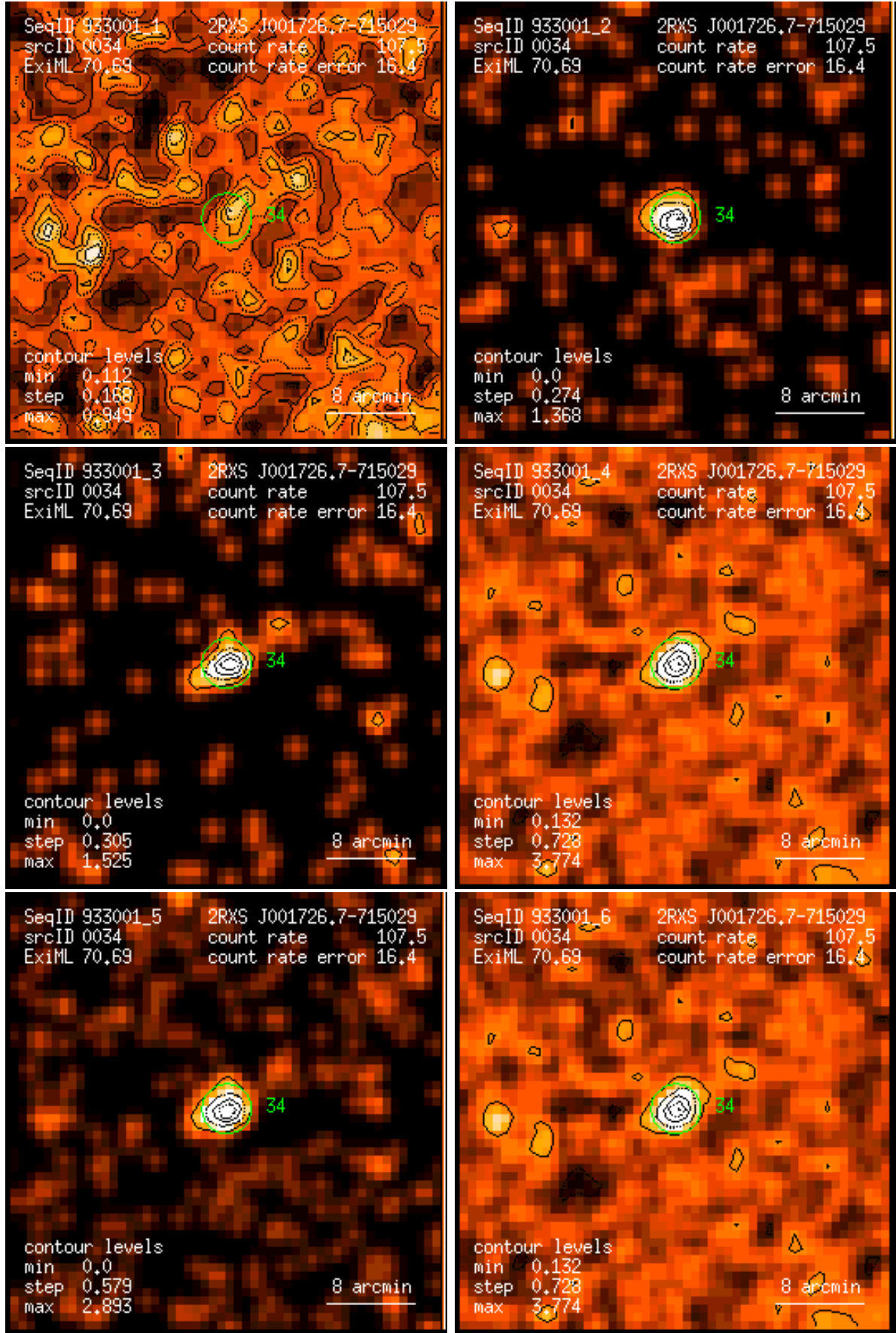
Figure 34: RASS 933001: detection 0034: band rate images, Gaussian filter: (1) PSPC channels 11 – 41, (2) 52 – 90, (3) 91 – 201, (4) 11 – 235, (5) 52 – 201, (6) 11 – 201. Broad band rates in counts/ks. Band rate contour levels in counts/ks/arcmin 2 .
