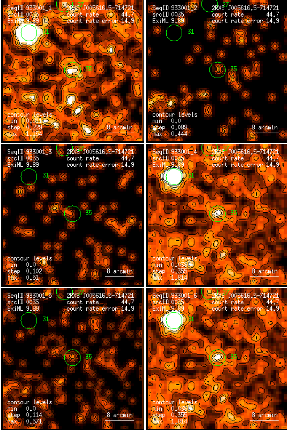
Figure 35: RASS 933001: detection 0035: band rate images, Gaussian filter: (1) PSPC channels 11 – 41, (2) 52 – 90, (3) 91 – 201, (4) 11 – 235, (5) 52 – 201, (6) 11 – 201. Broad band rates in counts/ks. Band rate contour levels in counts/ks/arcmin 2 .
