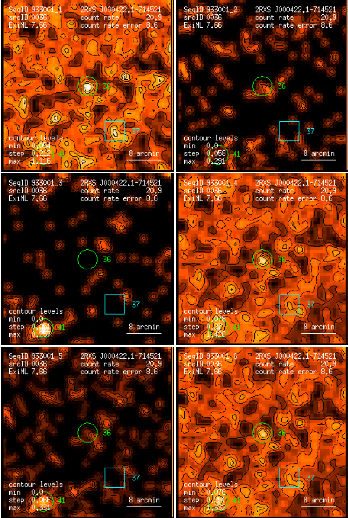
Figure 36: RASS 933001: detection 0036: band rate images, Gaussian filter: (1) PSPC channels 11 – 41, (2) 52 – 90, (3) 91 – 201, (4) 11 – 235, (5) 52 – 201, (6) 11 – 201. Broad band rates in counts/ks. Band rate contour levels in counts/ks/arcmin 2 .
