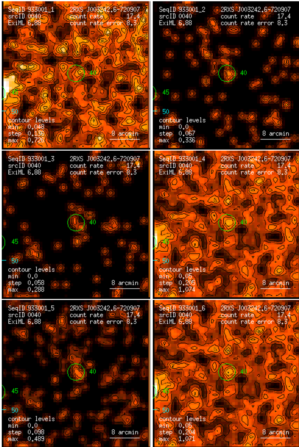
Figure 40: RASS 933001: detection 0040: band rate images, Gaussian filter: (1) PSPC channels 11 – 41, (2) 52 – 90, (3) 91 – 201, (4) 11 – 235, (5) 52 – 201, (6) 11 – 201. Broad band rates in counts/ks. Band rate contour levels in counts/ks/arcmin 2 .
