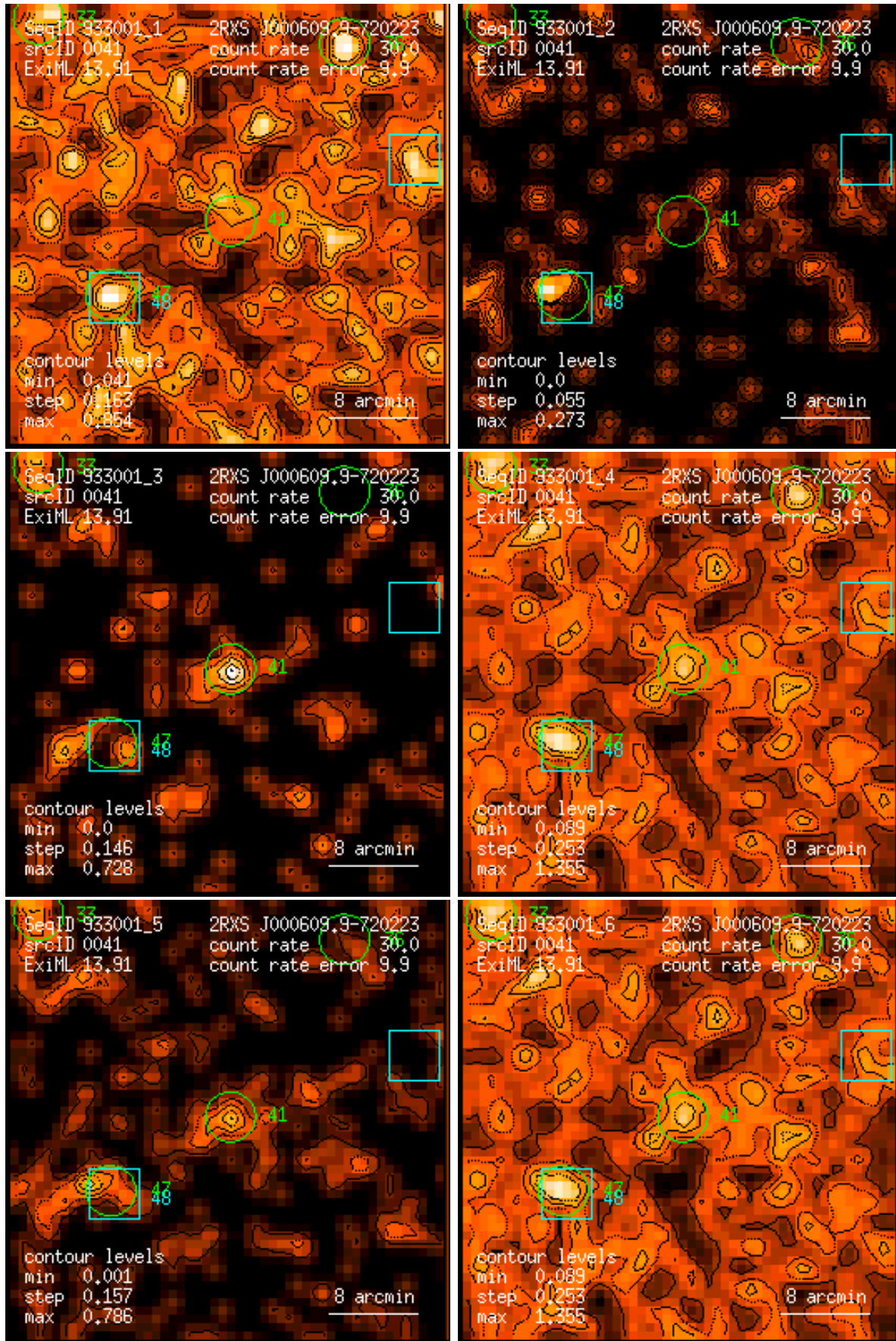
Figure 41: RASS 933001: detection 0041: band rate images, Gaussian filter: (1) PSPC channels 11 – 41, (2) 52 – 90, (3) 91 – 201, (4) 11 – 235, (5) 52 – 201, (6) 11 – 201. Broad band rates in counts/ks. Band rate contour levels in counts/ks/arcmin 2 .
