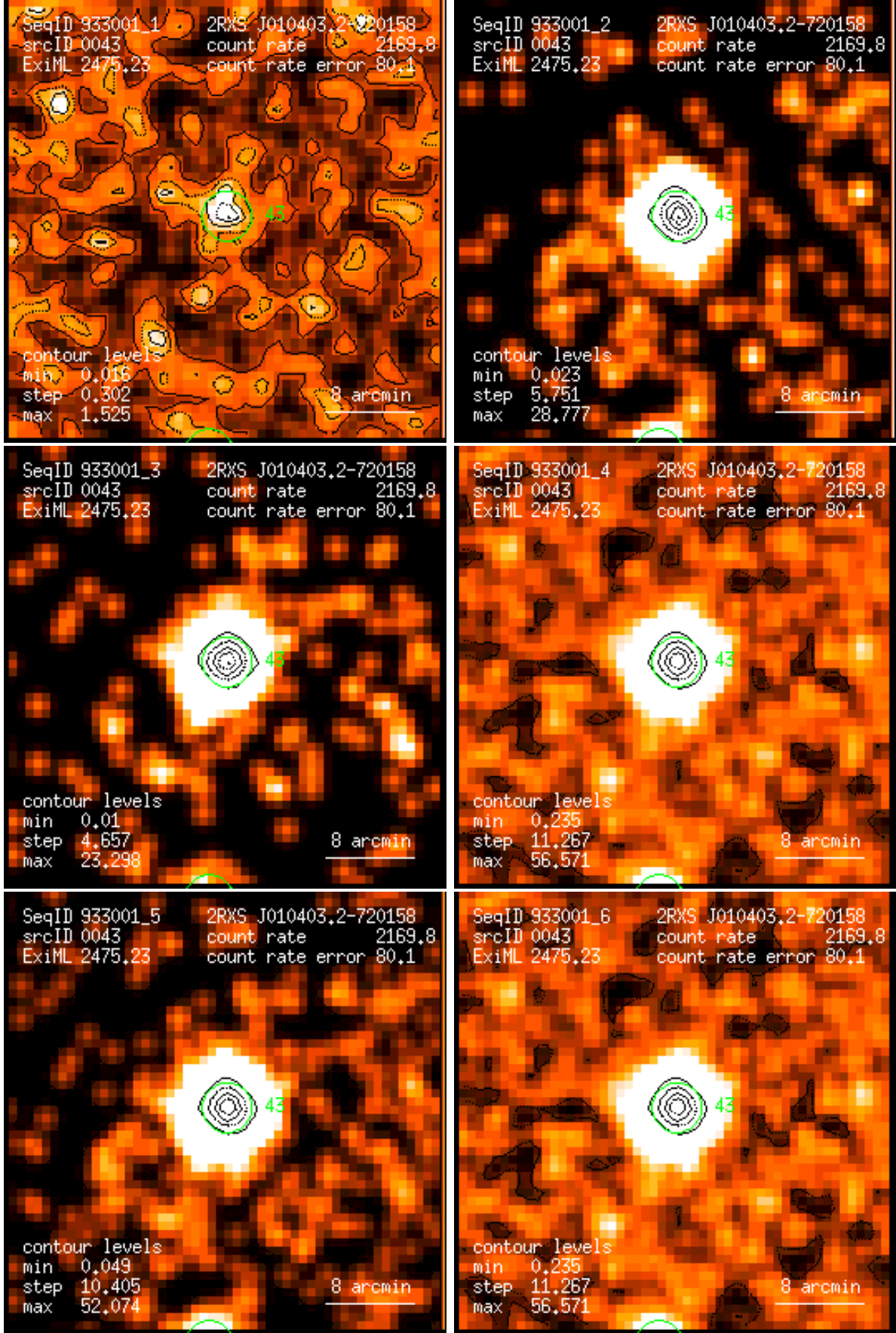
Figure 43: RASS 933001: detection 0043: band rate images, Gaussian filter: (1) PSPC channels 11 – 41, (2) 52 – 90, (3) 91 – 201, (4) 11 – 235, (5) 52 – 201, (6) 11 – 201. Broad band rates in counts/ks. Band rate contour levels in counts/ks/arcmin 2 .
