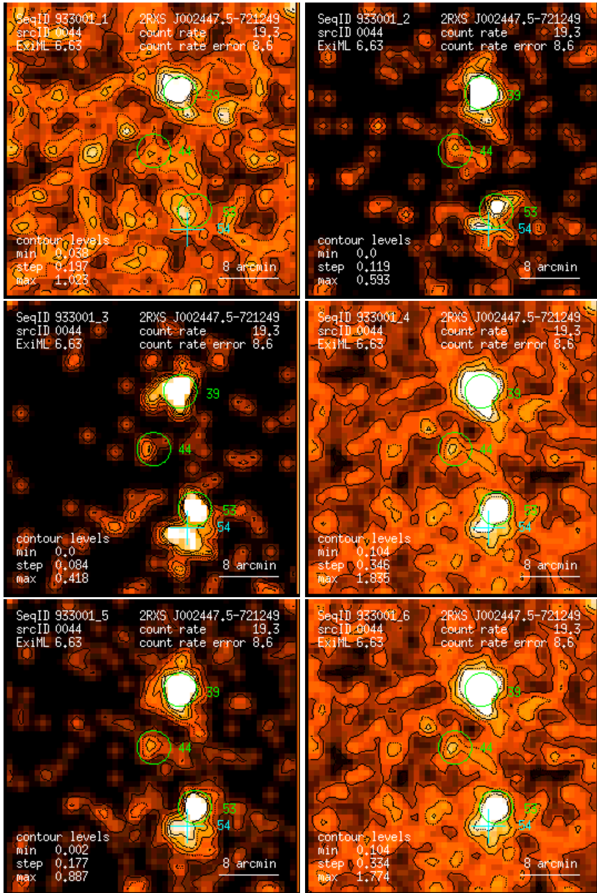
Figure 44: RASS 933001: detection 0044: band rate images, Gaussian filter: (1) PSPC channels 11 – 41, (2) 52 – 90, (3) 91 – 201, (4) 11 – 235, (5) 52 – 201, (6) 11 – 201. Broad band rates in counts/ks. Band rate contour levels in counts/ks/arcmin 2 .
