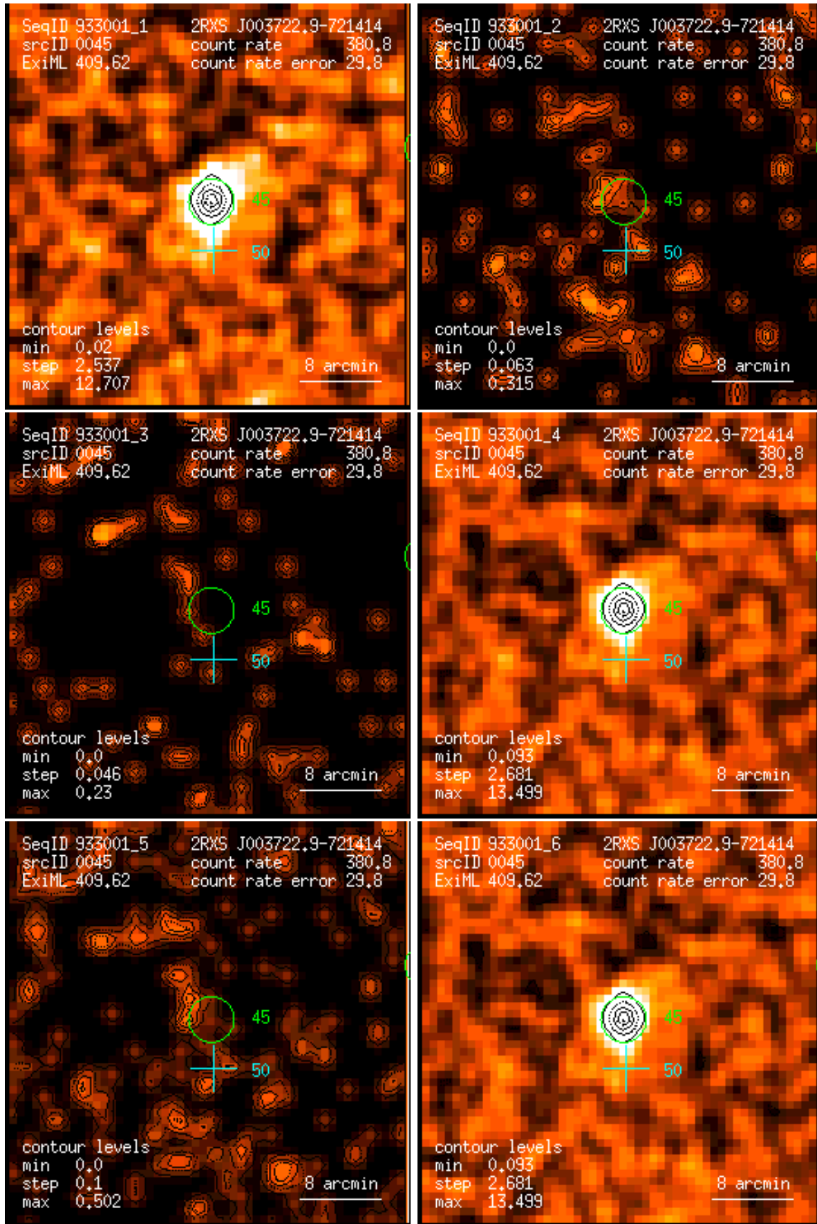
Figure 45: RASS 933001: detection 0045: band rate images, Gaussian filter: (1) PSPC channels 11 – 41, (2) 52 – 90, (3) 91 – 201, (4) 11 – 235, (5) 52 – 201, (6) 11 – 201. Broad band rates in counts/ks. Band rate contour levels in counts/ks/arcmin 2 .
