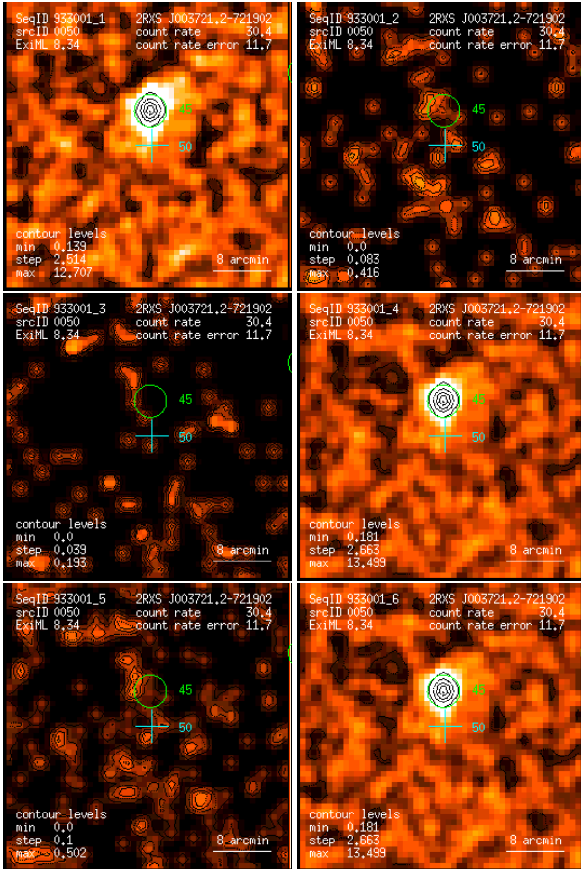
Figure 50: RASS 933001: detection 0050: band rate images, Gaussian filter: (1) PSPC channels 11 – 41, (2) 52 – 90, (3) 91 – 201, (4) 11 – 235, (5) 52 – 201, (6) 11 – 201. Broad band rates in counts/ks. Band rate contour levels in counts/ks/arcmin 2 .
