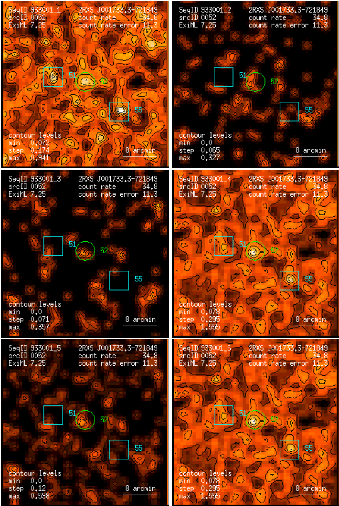
Figure 52: RASS 933001: detection 0052: band rate images, Gaussian filter: (1) PSPC channels 11 – 41, (2) 52 – 90, (3) 91 – 201, (4) 11 – 235, (5) 52 – 201, (6) 11 – 201. Broad band rates in counts/ks. Band rate contour levels in counts/ks/arcmin 2 .
