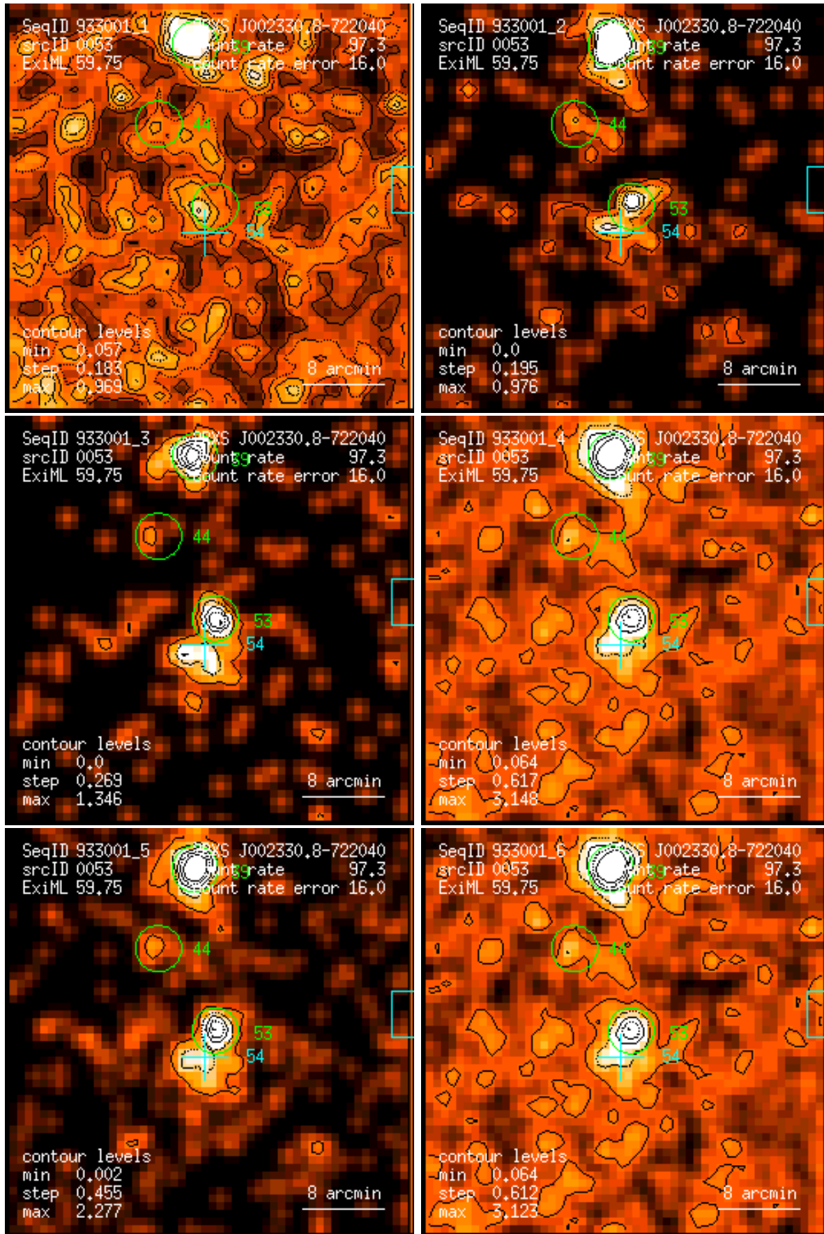
Figure 53: RASS 933001: detection 0053: band rate images, Gaussian filter: (1) PSPC channels 11 – 41, (2) 52 – 90, (3) 91 – 201, (4) 11 – 235, (5) 52 – 201, (6) 11 – 201. Broad band rates in counts/ks. Band rate contour levels in counts/ks/arcmin 2 .
