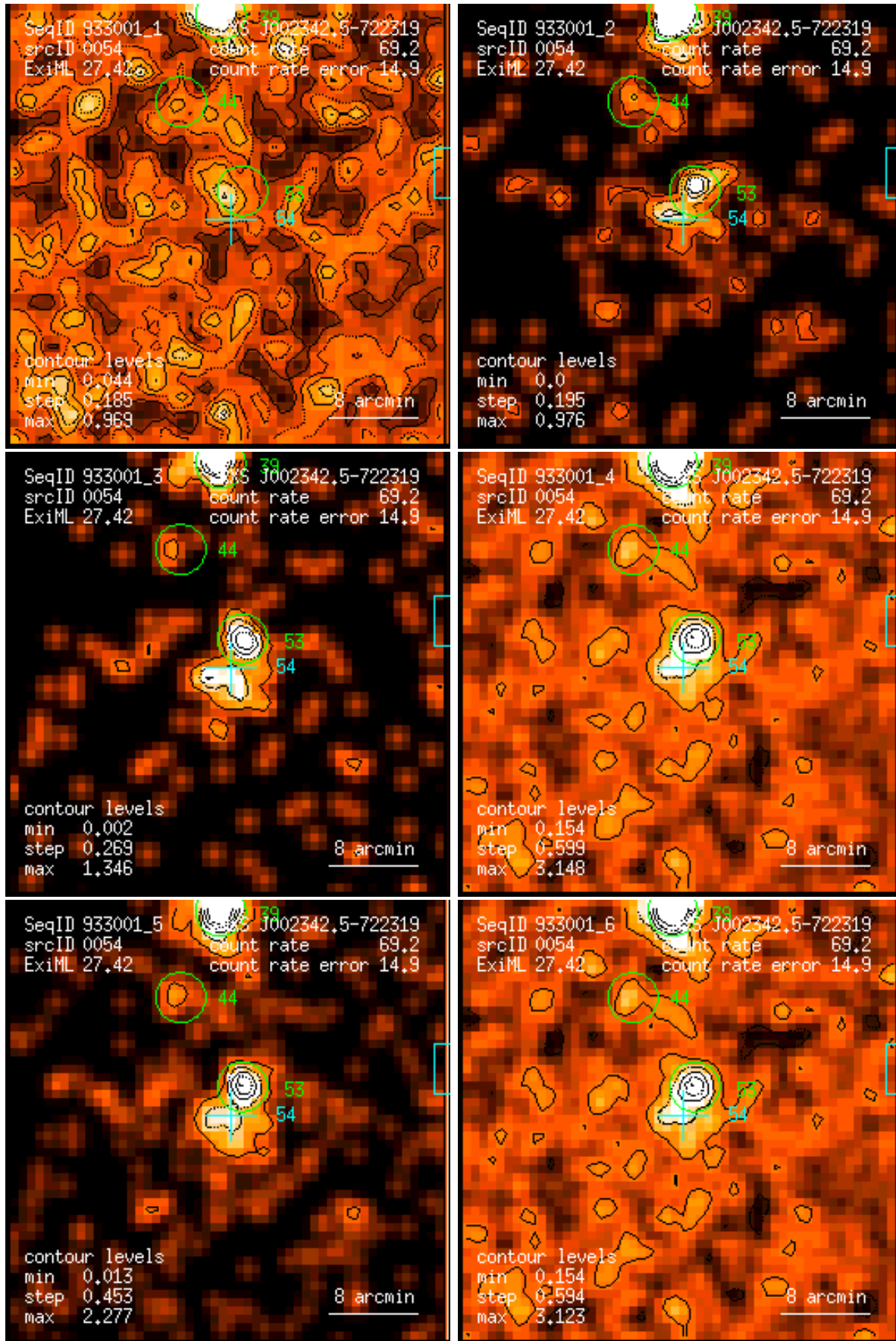
Figure 54: RASS 933001: detection 0054: band rate images, Gaussian filter: (1) PSPC channels 11 – 41, (2) 52 – 90, (3) 91 – 201, (4) 11 – 235, (5) 52 – 201, (6) 11 – 201. Broad band rates in counts/ks. Band rate contour levels in counts/ks/arcmin 2 .
