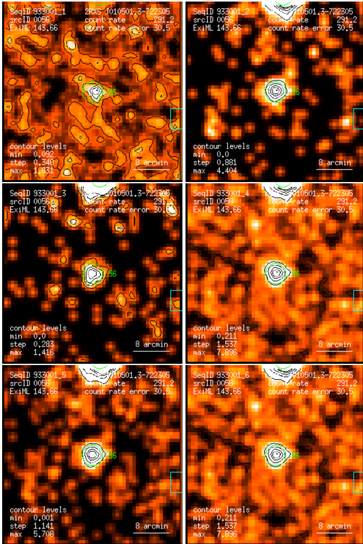
Figure 56: RASS 933001: detection 0056: band rate images, Gaussian filter: (1) PSPC channels 11 – 41, (2) 52 – 90, (3) 91 – 201, (4) 11 – 235, (5) 52 – 201, (6) 11 – 201. Broad band rates in counts/ks. Band rate contour levels in counts/ks/arcmin 2 .
