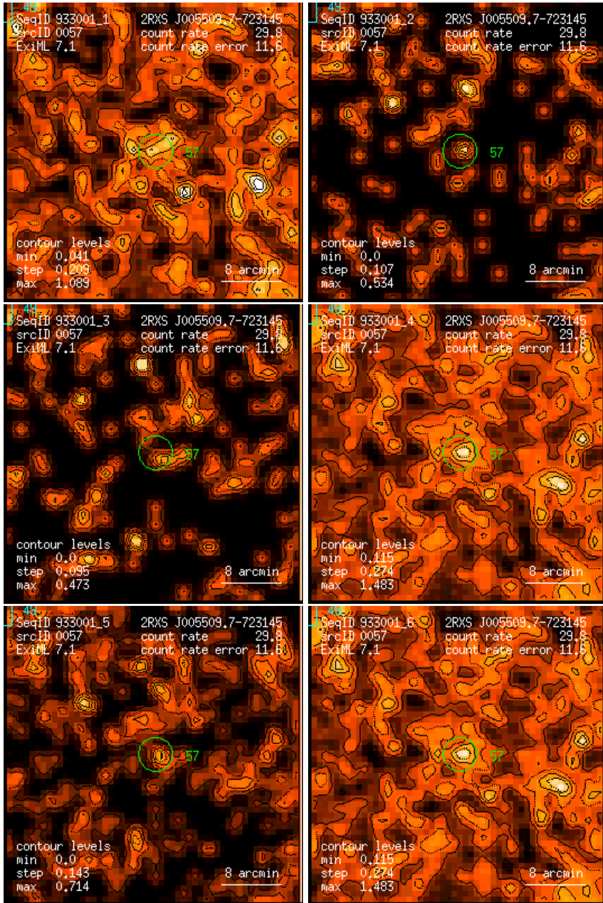
Figure 57: RASS 933001: detection 0057: band rate images, Gaussian filter: (1) PSPC channels 11 – 41, (2) 52 – 90, (3) 91 – 201, (4) 11 – 235, (5) 52 – 201, (6) 11 – 201. Broad band rates in counts/ks. Band rate contour levels in counts/ks/arcmin 2 .
