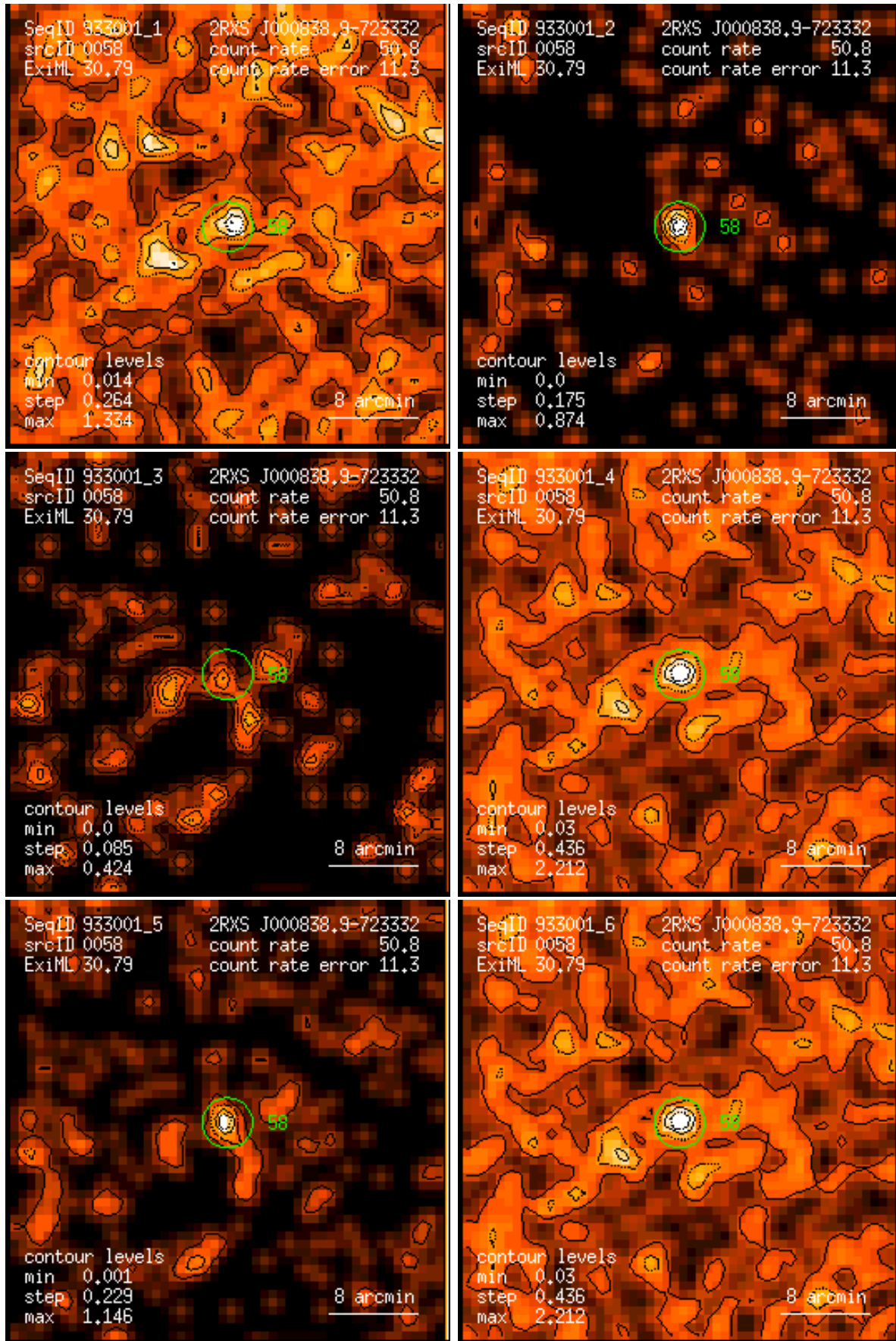
Figure 58: RASS 933001: detection 0058: band rate images, Gaussian filter: (1) PSPC channels 11 – 41, (2) 52 – 90, (3) 91 – 201, (4) 11 – 235, (5) 52 – 201, (6) 11 – 201. Broad band rates in counts/ks. Band rate contour levels in counts/ks/arcmin 2 .
