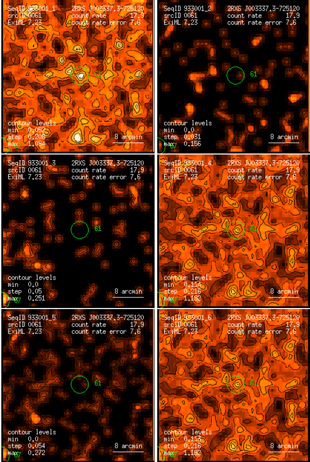
Figure 61: RASS 933001: detection 0061: band rate images, Gaussian filter: (1) PSPC channels 11 – 41, (2) 52 – 90, (3) 91 – 201, (4) 11 – 235, (5) 52 – 201, (6) 11 – 201. Broad band rates in counts/ks. Band rate contour levels in counts/ks/arcmin 2 .
