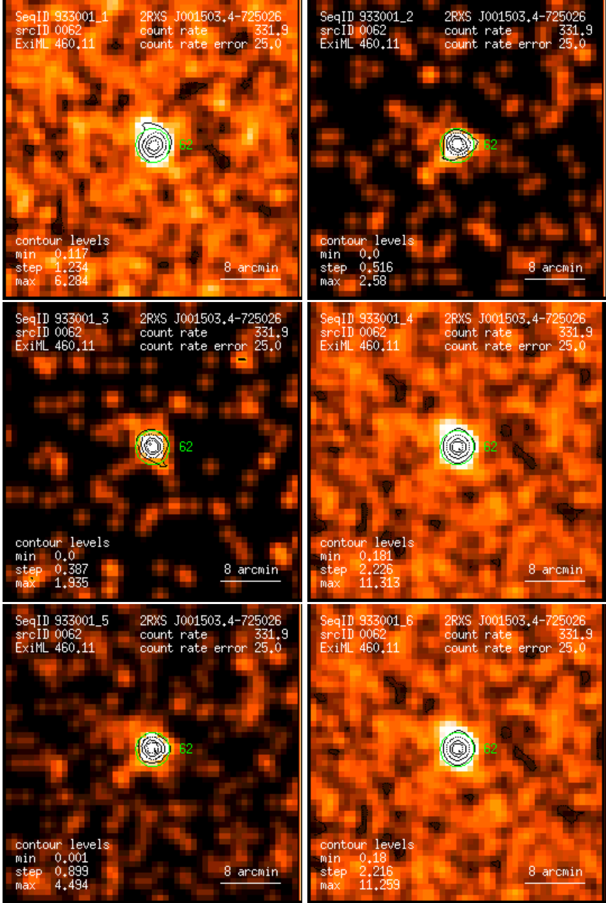
Figure 62: RASS 933001: detection 0062: band rate images, Gaussian filter: (1) PSPC channels 11 – 41, (2) 52 – 90, (3) 91 – 201, (4) 11 – 235, (5) 52 – 201, (6) 11 – 201. Broad band rates in counts/ks. Band rate contour levels in counts/ks/arcmin 2 .
