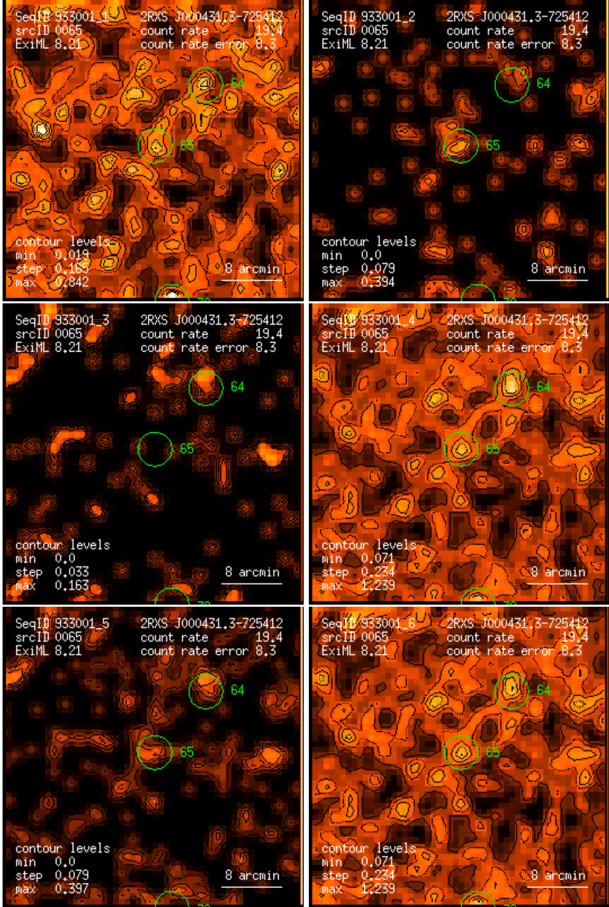
Figure 65: RASS 933001: detection 0065: band rate images, Gaussian filter: (1) PSPC channels 11 – 41, (2) 52 – 90, (3) 91 – 201, (4) 11 – 235, (5) 52 – 201, (6) 11 – 201. Broad band rates in counts/ks. Band rate contour levels in counts/ks/arcmin 2 .
