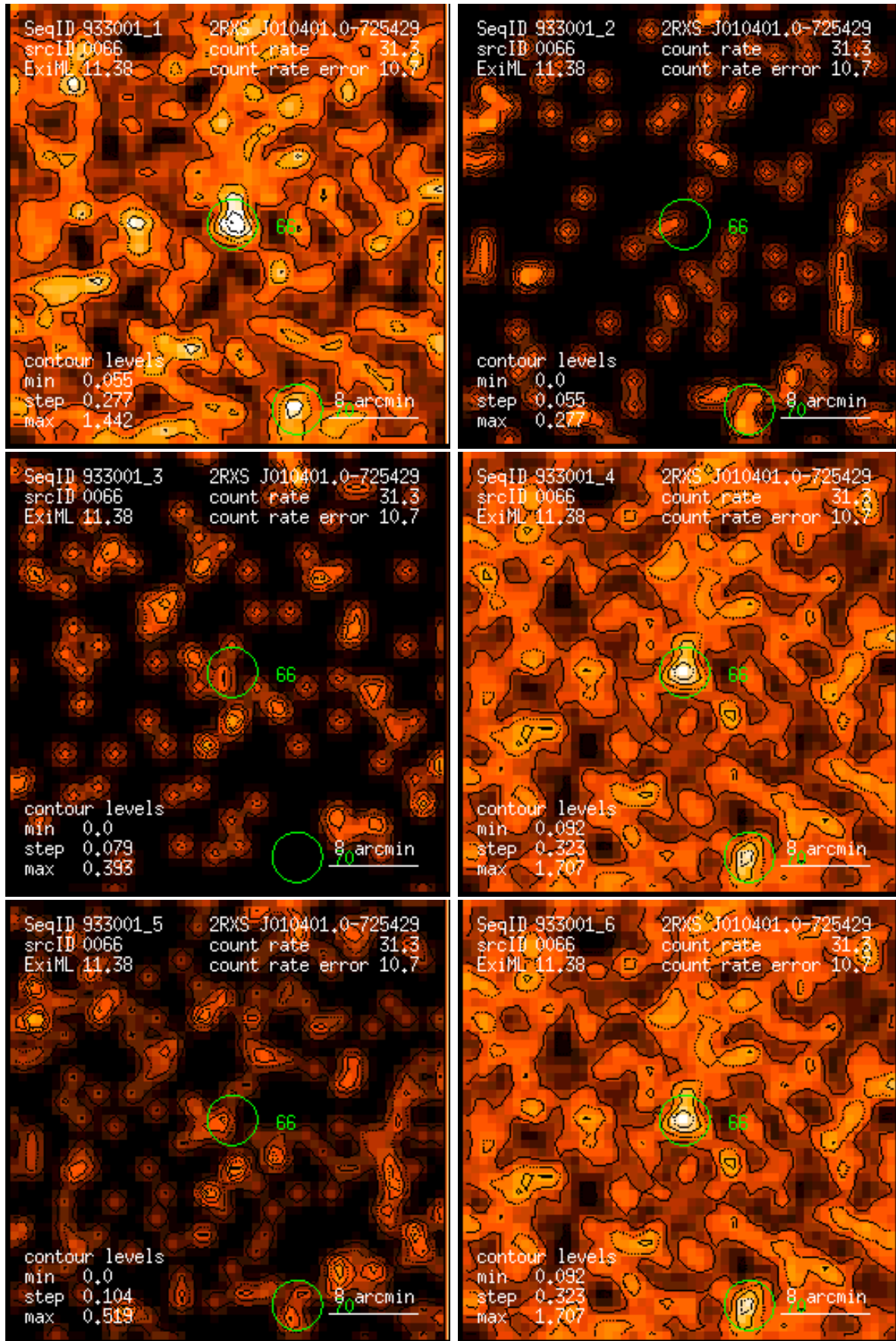
Figure 66: RASS 933001: detection 0066: band rate images, Gaussian filter: (1) PSPC channels 11 – 41, (2) 52 – 90, (3) 91 – 201, (4) 11 – 235, (5) 52 – 201, (6) 11 – 201. Broad band rates in counts/ks. Band rate contour levels in counts/ks/arcmin 2 .
