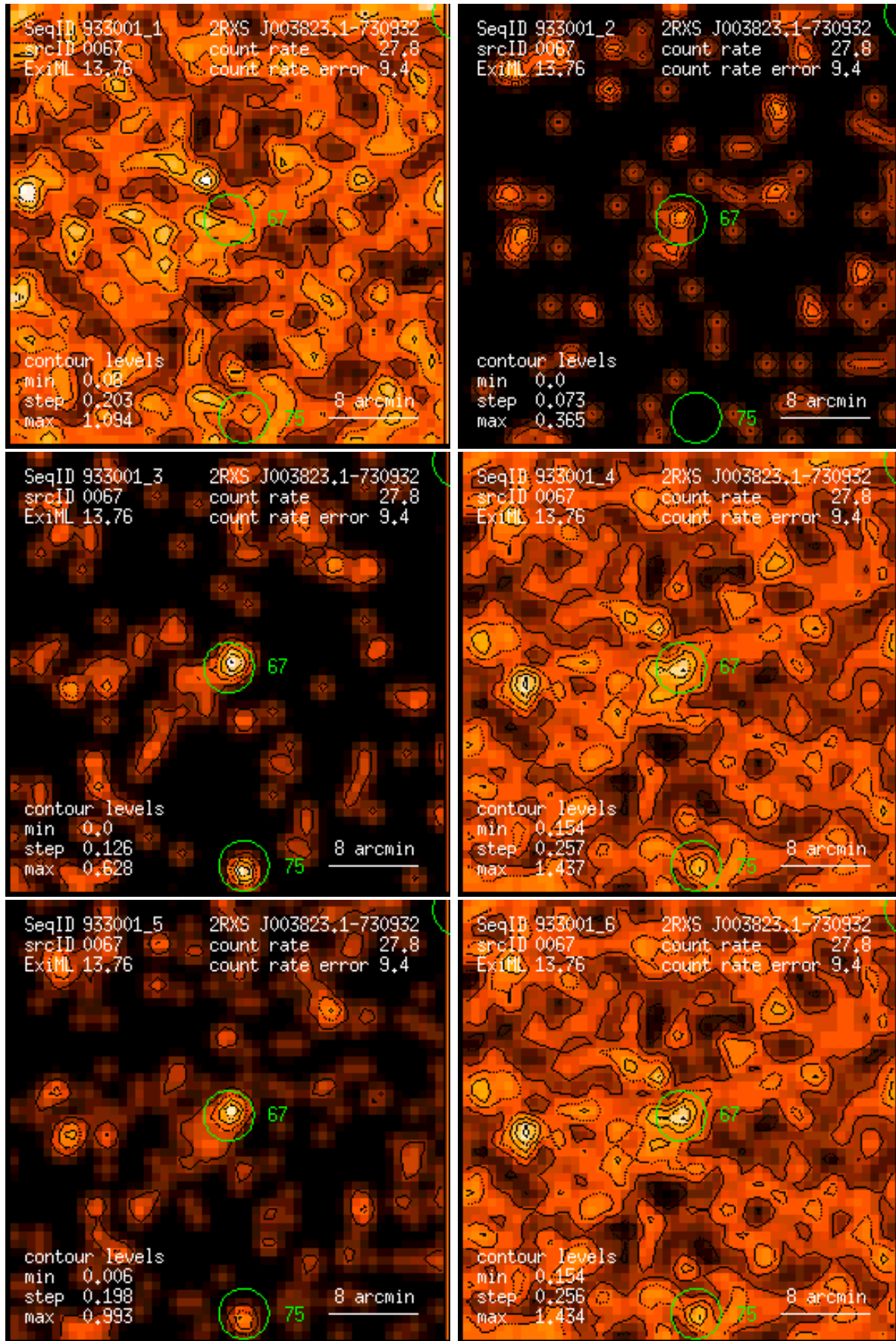
Figure 67: RASS 933001: detection 0067: band rate images, Gaussian filter: (1) PSPC channels 11 – 41, (2) 52 – 90, (3) 91 – 201, (4) 11 – 235, (5) 52 – 201, (6) 11 – 201. Broad band rates in counts/ks. Band rate contour levels in counts/ks/arcmin 2 .
