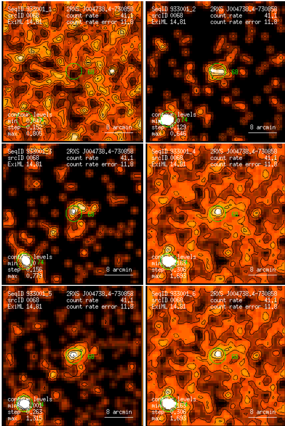
Figure 68: RASS 933001: detection 0068: band rate images, Gaussian filter: (1) PSPC channels 11 – 41, (2) 52 – 90, (3) 91 – 201, (4) 11 – 235, (5) 52 – 201, (6) 11 – 201. Broad band rates in counts/ks. Band rate contour levels in counts/ks/arcmin 2 .
