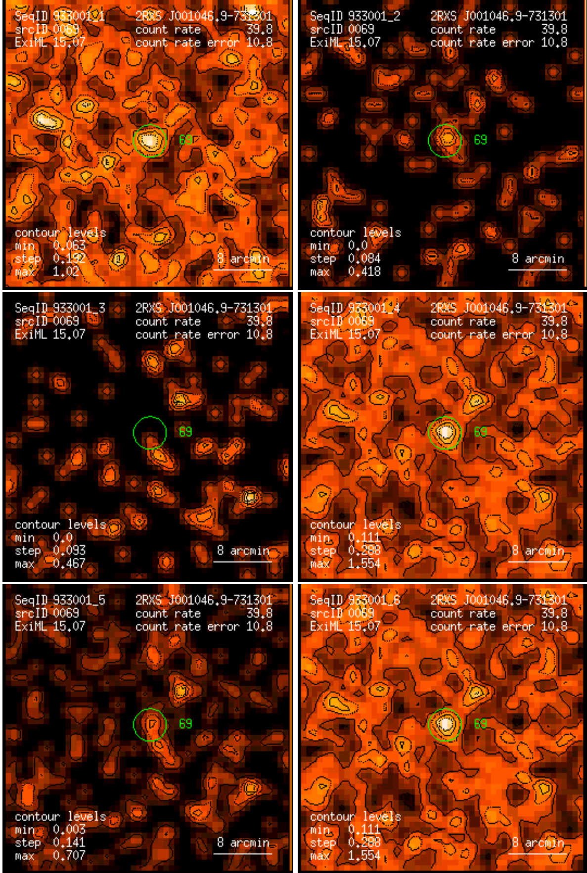
Figure 69: RASS 933001: detection 0069: band rate images, Gaussian filter: (1) PSPC channels 11 – 41, (2) 52 – 90, (3) 91 – 201, (4) 11 – 235, (5) 52 – 201, (6) 11 – 201. Broad band rates in counts/ks. Band rate contour levels in counts/ks/arcmin 2 .
