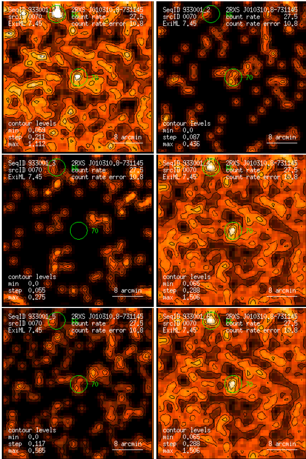
Figure 70: RASS 933001: detection 0070: band rate images, Gaussian filter: (1) PSPC channels 11 – 41, (2) 52 – 90, (3) 91 – 201, (4) 11 – 235, (5) 52 – 201, (6) 11 – 201. Broad band rates in counts/ks. Band rate contour levels in counts/ks/arcmin 2 .
