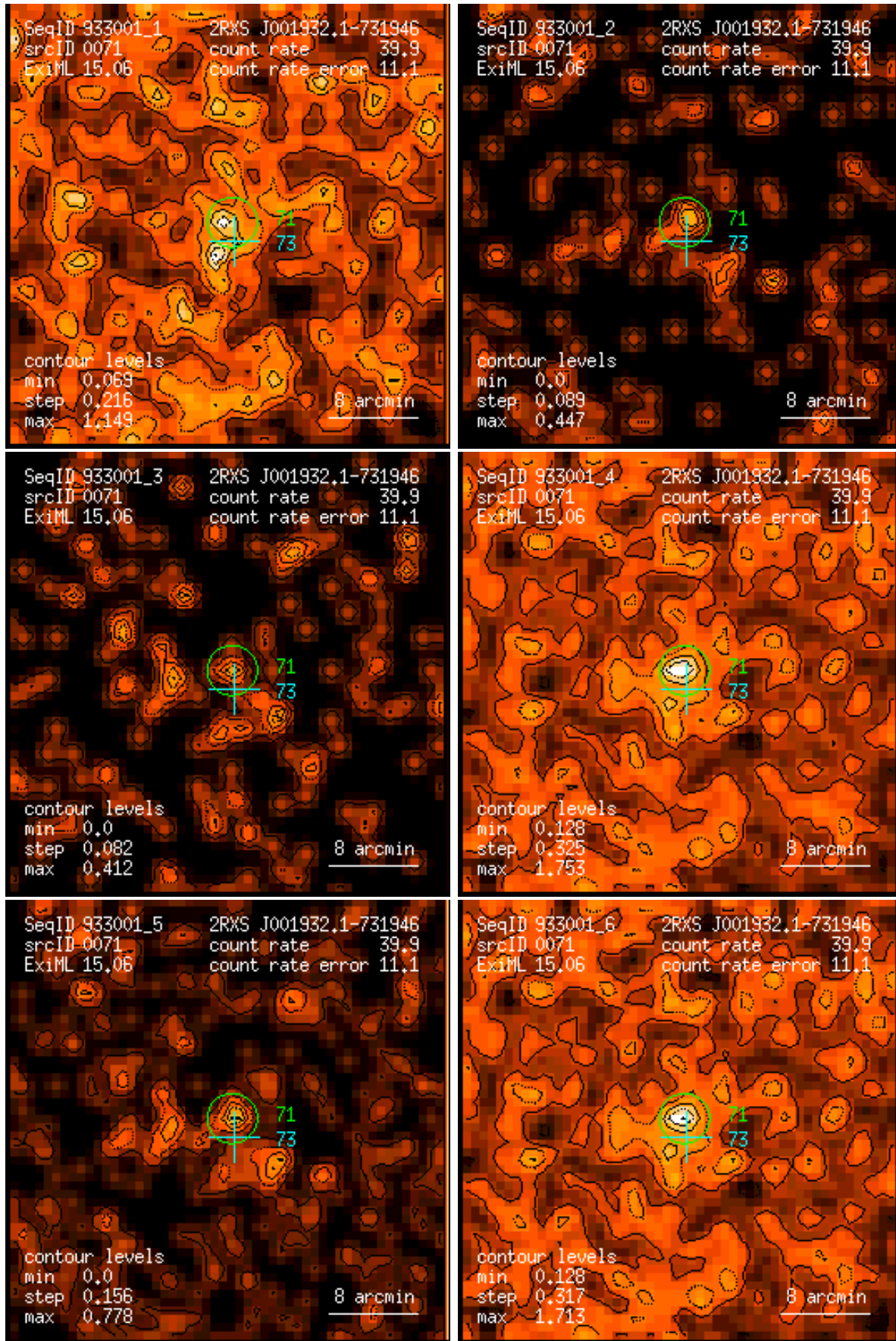
Figure 71: RASS 933001: detection 0071: band rate images, Gaussian filter: (1) PSPC channels 11 – 41, (2) 52 – 90, (3) 91 – 201, (4) 11 – 235, (5) 52 – 201, (6) 11 – 201. Broad band rates in counts/ks. Band rate contour levels in counts/ks/arcmin 2 .
