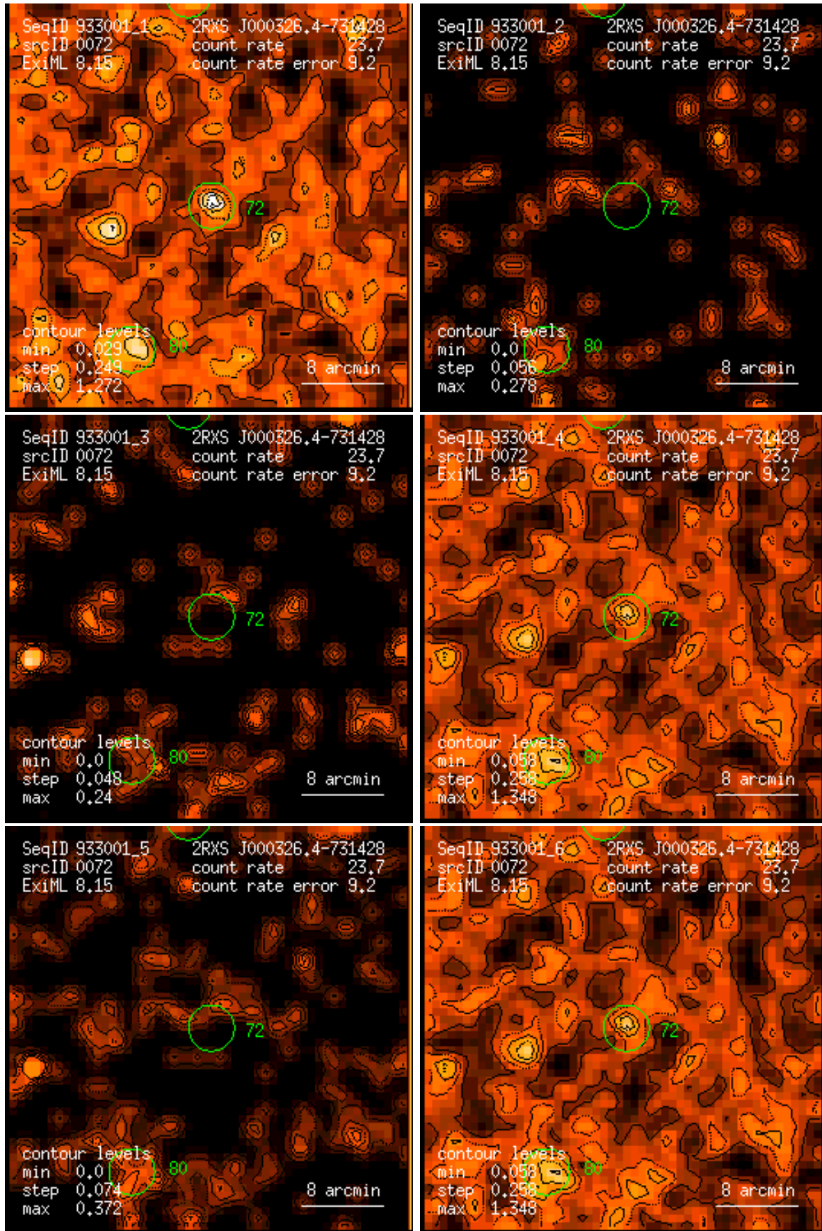
Figure 72: RASS 933001: detection 0072: band rate images, Gaussian filter: (1) PSPC channels 11 – 41, (2) 52 – 90, (3) 91 – 201, (4) 11 – 235, (5) 52 – 201, (6) 11 – 201. Broad band rates in counts/ks. Band rate contour levels in counts/ks/arcmin 2 .
