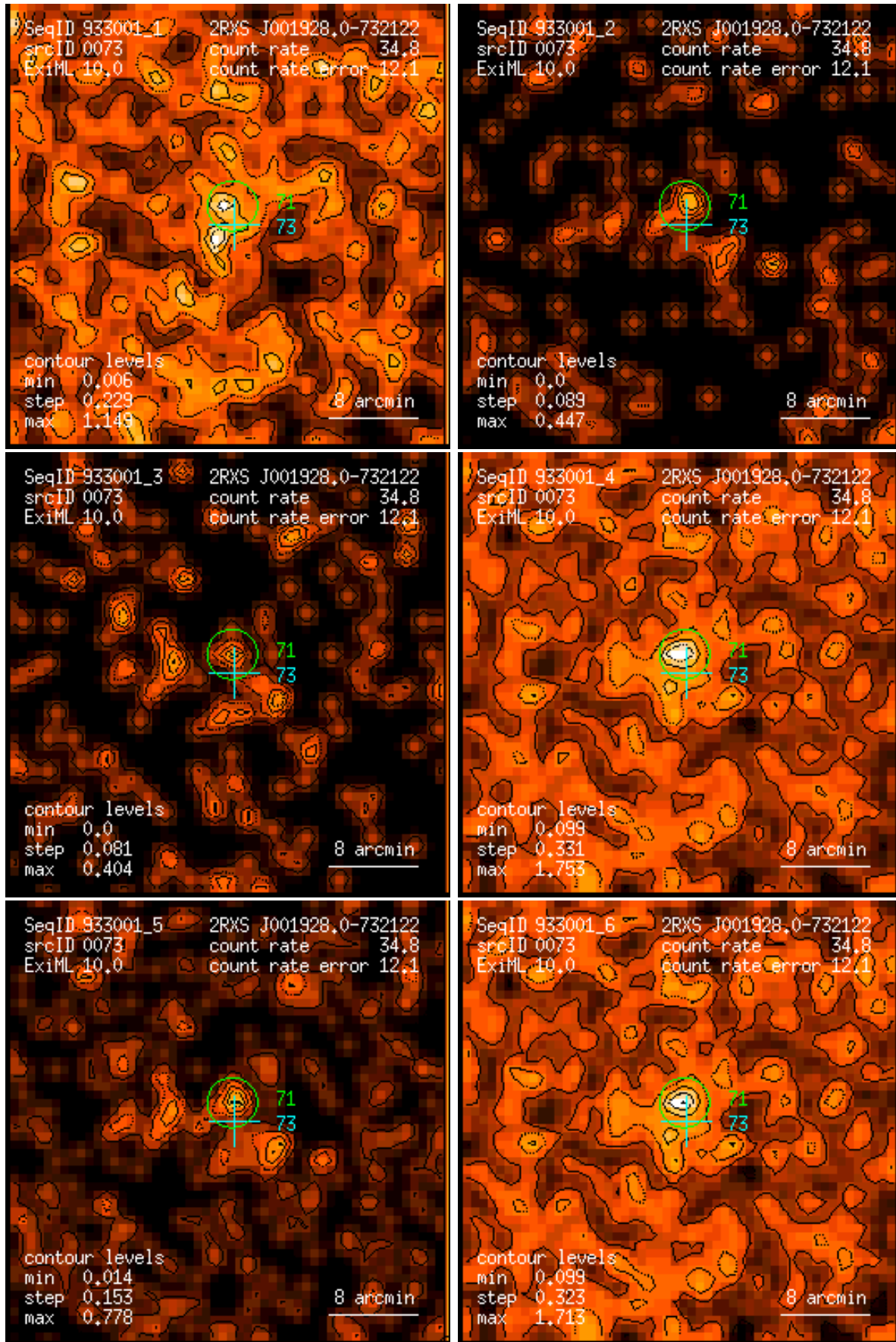
Figure 73: RASS 933001: detection 0073: band rate images, Gaussian filter: (1) PSPC channels 11 – 41, (2) 52 – 90, (3) 91 – 201, (4) 11 – 235, (5) 52 – 201, (6) 11 – 201. Broad band rates in counts/ks. Band rate contour levels in counts/ks/arcmin 2 .
