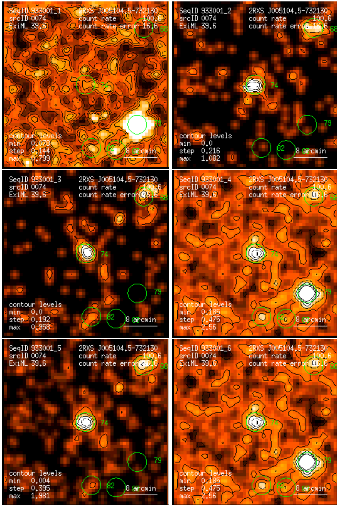
Figure 74: RASS 933001: detection 0074: band rate images, Gaussian filter: (1) PSPC channels 11 – 41, (2) 52 – 90, (3) 91 – 201, (4) 11 – 235, (5) 52 – 201, (6) 11 – 201. Broad band rates in counts/ks. Band rate contour levels in counts/ks/arcmin 2 .
