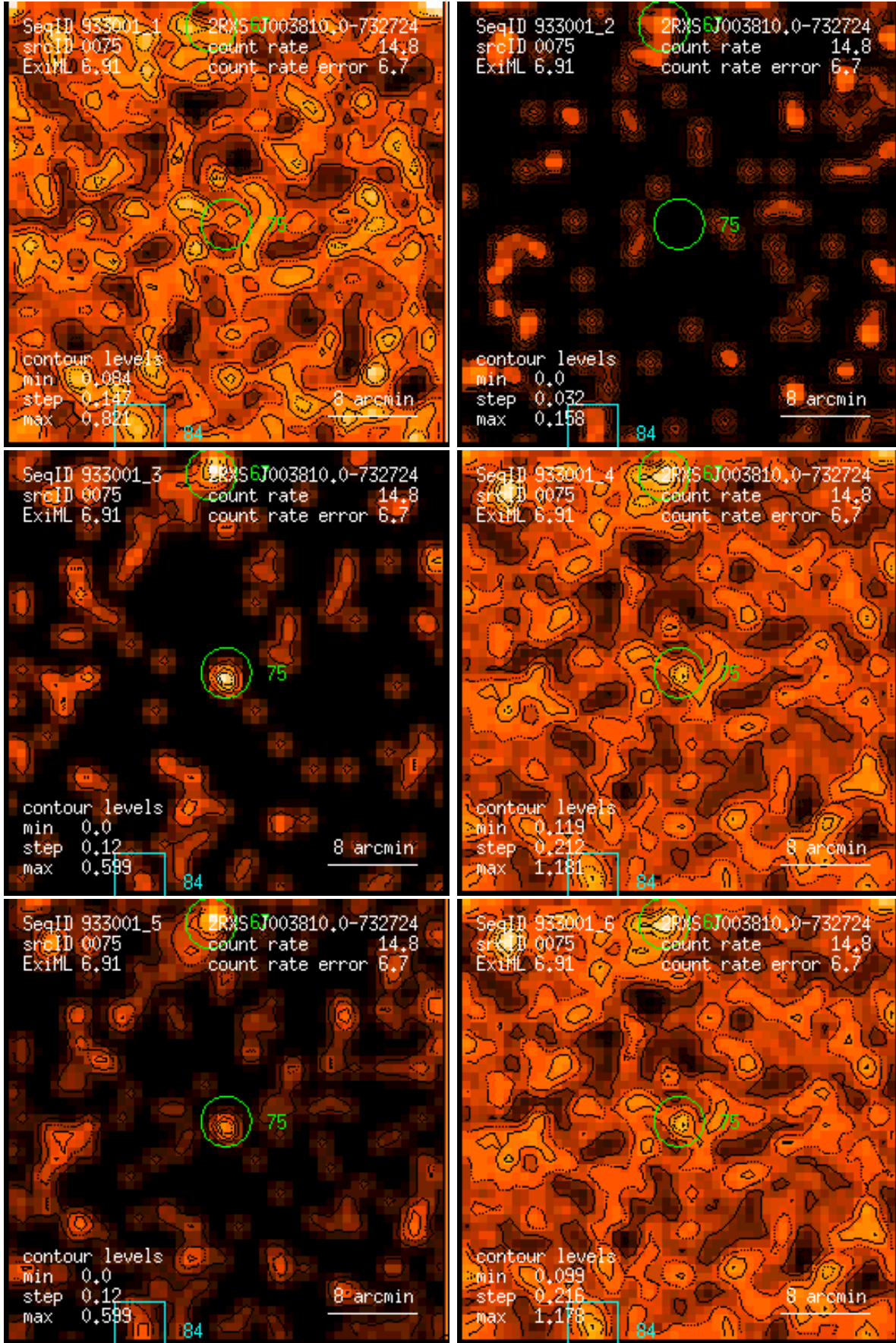
Figure 75: RASS 933001: detection 0075: band rate images, Gaussian filter: (1) PSPC channels 11 – 41, (2) 52 – 90, (3) 91 – 201, (4) 11 – 235, (5) 52 – 201, (6) 11 – 201. Broad band rates in counts/ks. Band rate contour levels in counts/ks/arcmin 2 .
