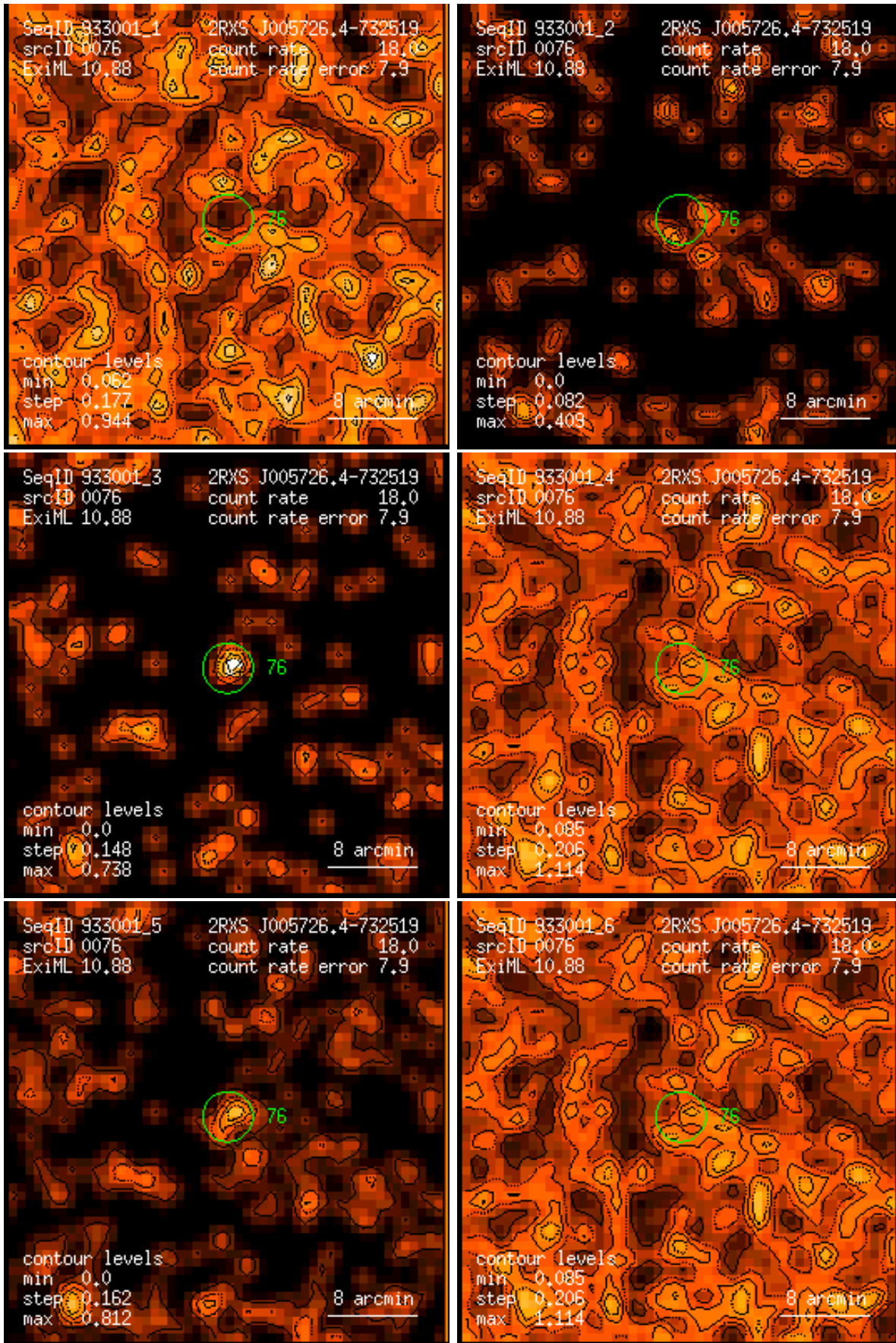
Figure 76: RASS 933001: detection 0076: band rate images, Gaussian filter: (1) PSPC channels 11 – 41, (2) 52 – 90, (3) 91 – 201, (4) 11 – 235, (5) 52 – 201, (6) 11 – 201. Broad band rates in counts/ks. Band rate contour levels in counts/ks/arcmin 2 .
