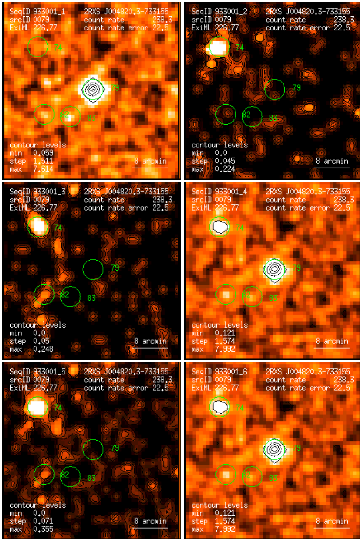
Figure 79: RASS 933001: detection 0079: band rate images, Gaussian filter: (1) PSPC channels 11 – 41, (2) 52 – 90, (3) 91 – 201, (4) 11 – 235, (5) 52 – 201, (6) 11 – 201. Broad band rates in counts/ks. Band rate contour levels in counts/ks/arcmin 2 .
